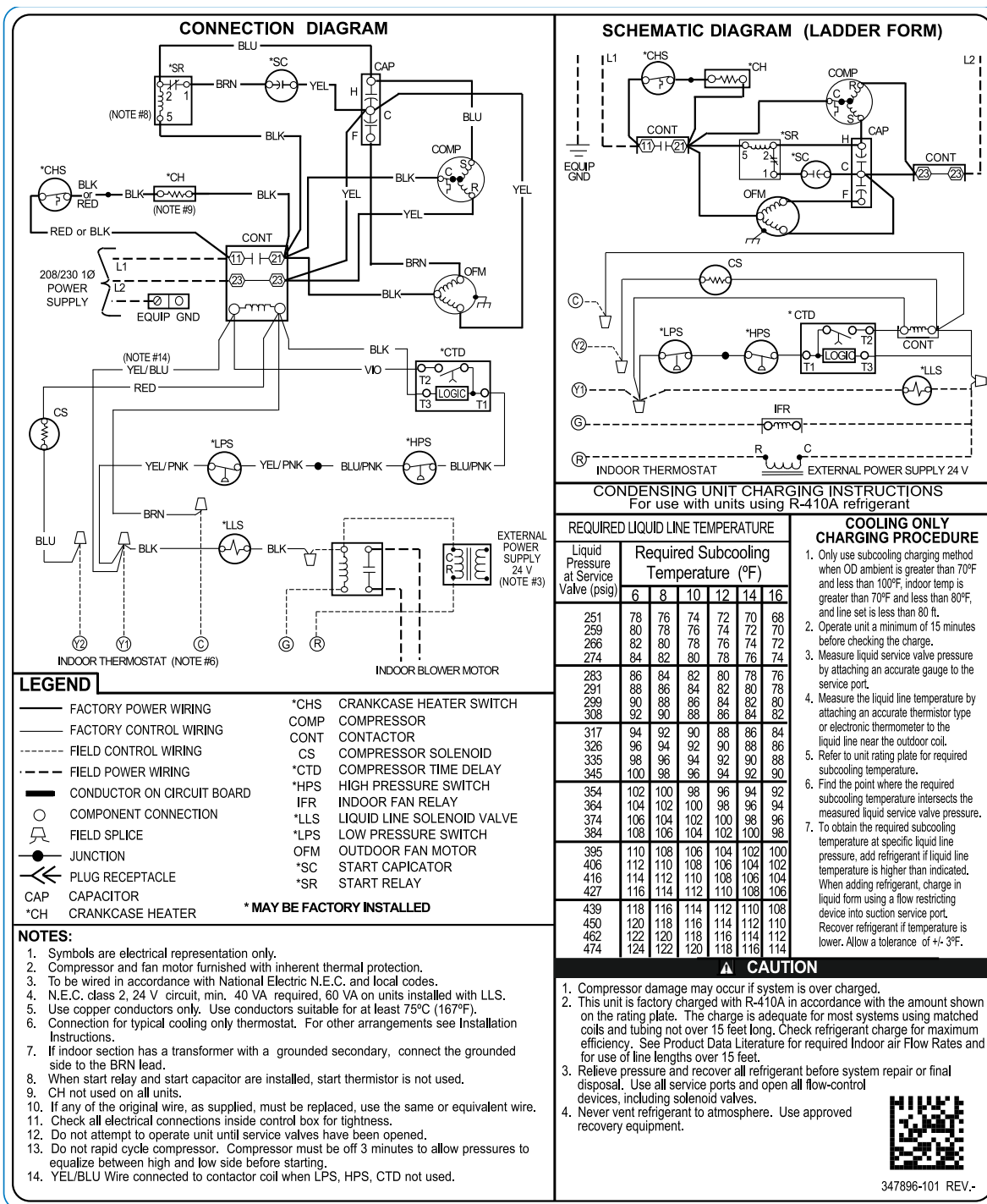
Fig. 1 – 208/230-1 - Model Sizes 24 - 60
