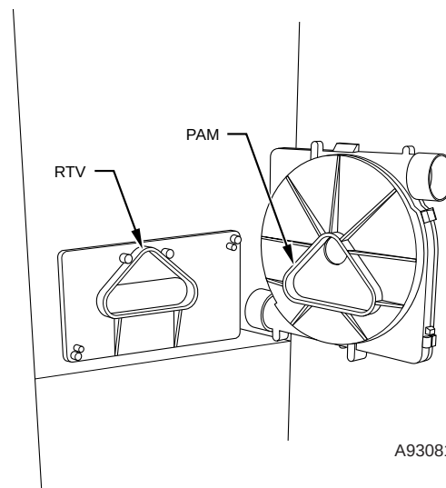
Fig. 2—Inducer Housing to Collector Box Gasket
