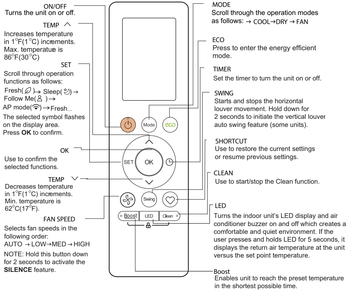
Fig. 7 — Remote Controller
