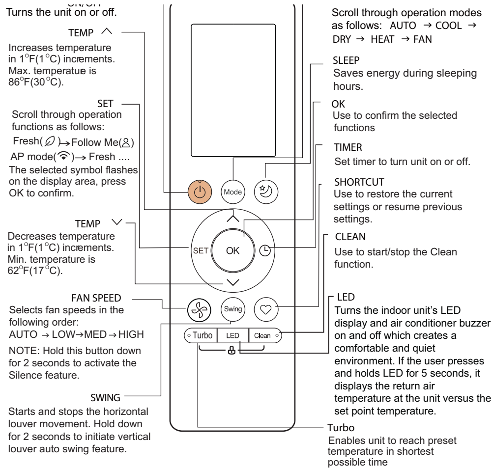
Fig. 5 — Remote Controller
