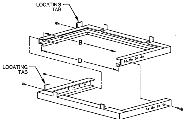
Disassembled
