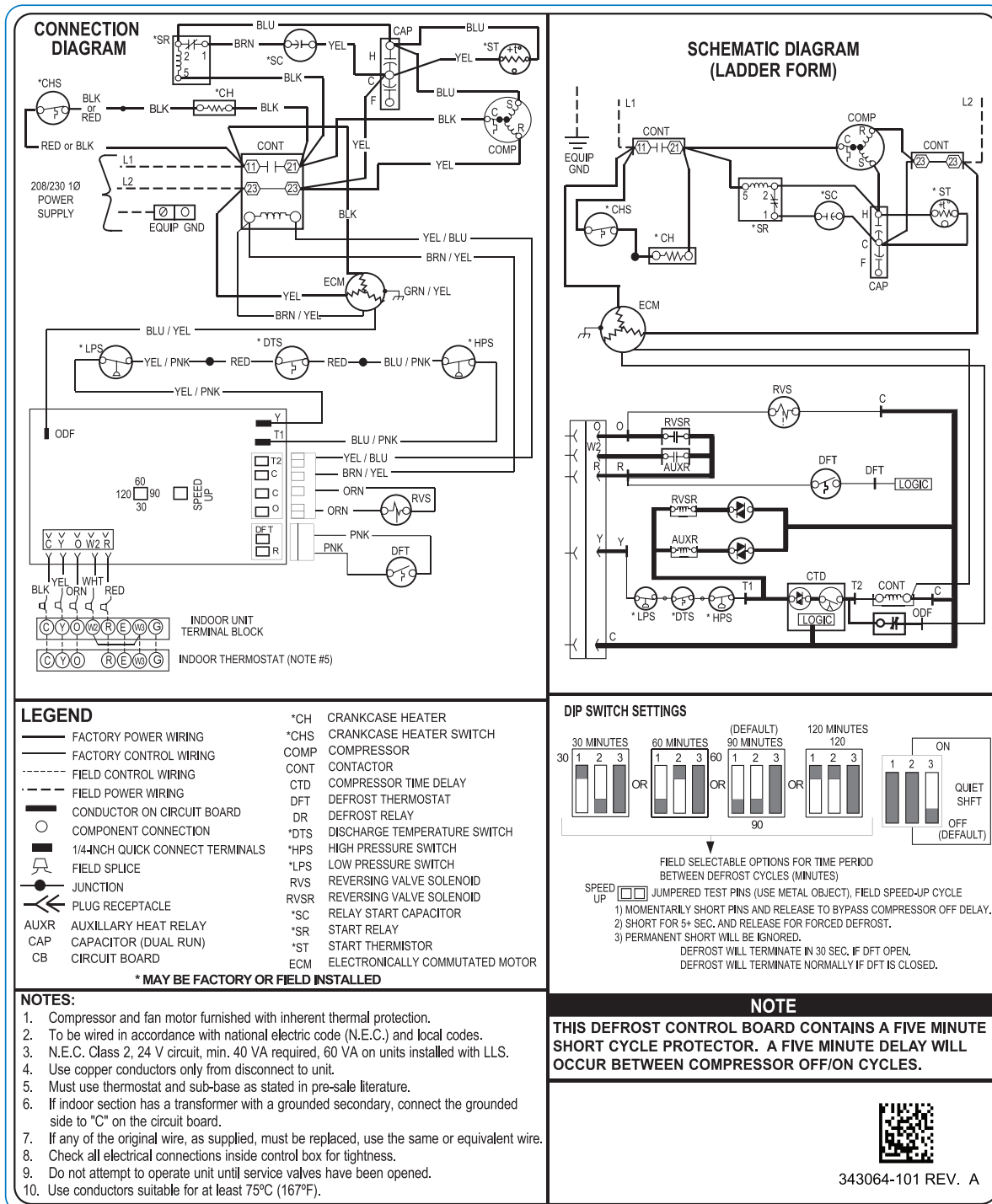
Fig. 2 – Wiring Diagram — Model sizes 42, 60 - 208/230-1
