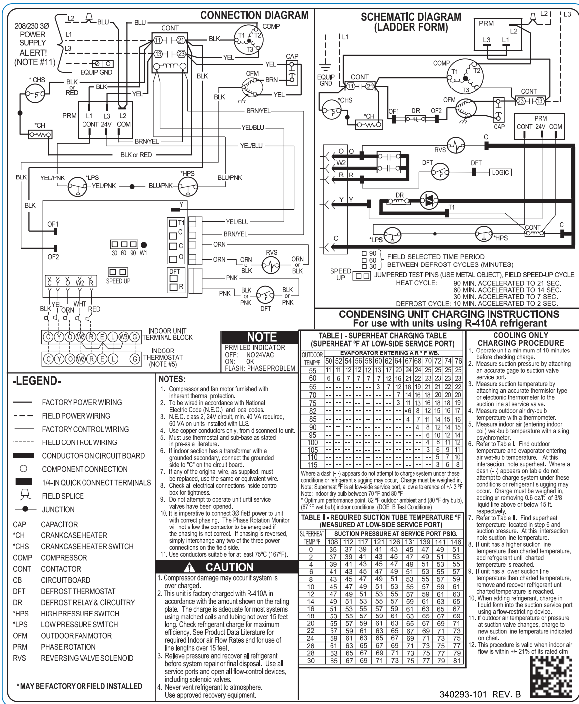
Fig. 3 – Wiring Diagram — Model sizes 36, 48 - 208/230-3
