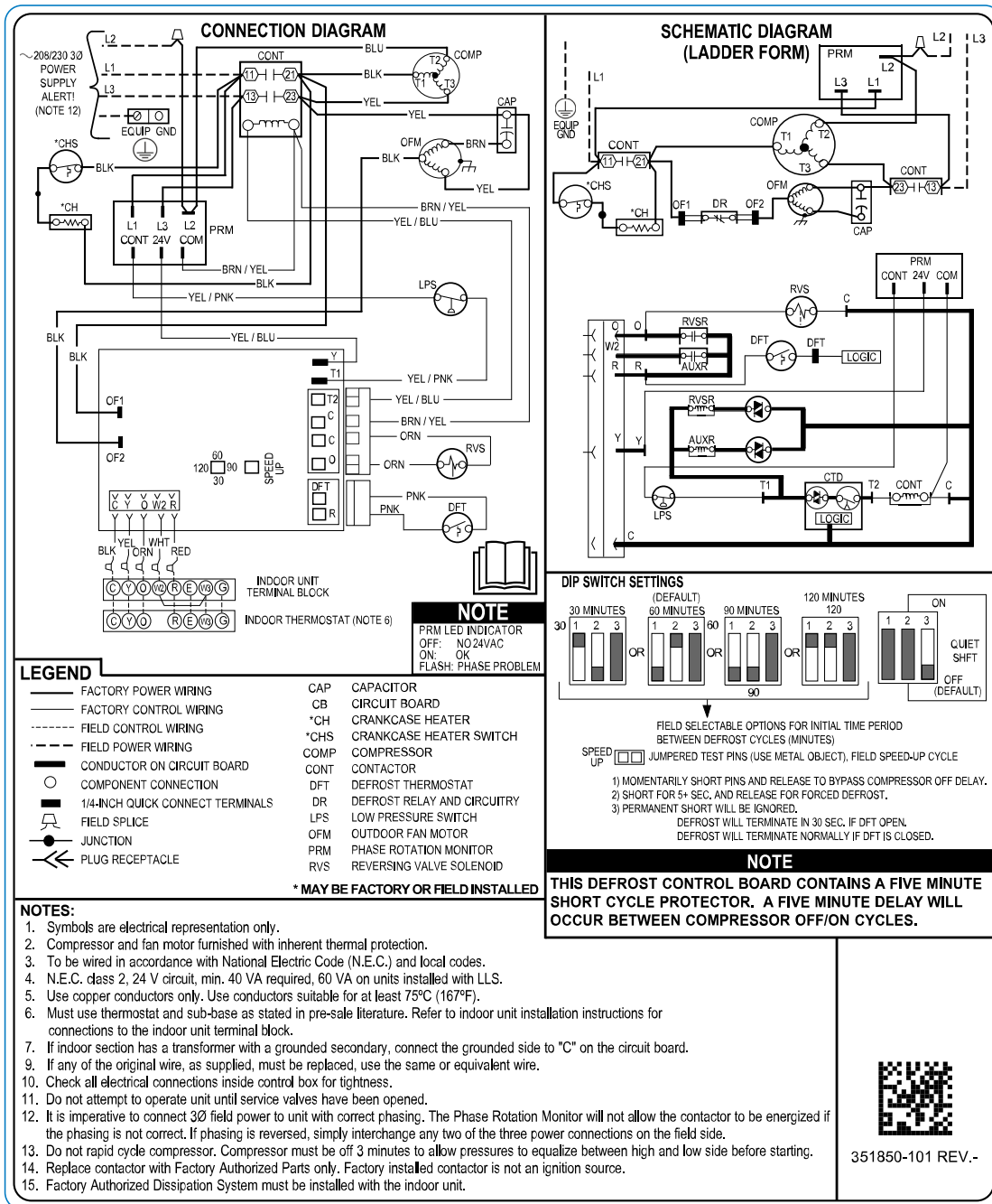
Fig. 2 – 208/230-3 Sizes (3, 4 and 5 Tons)
