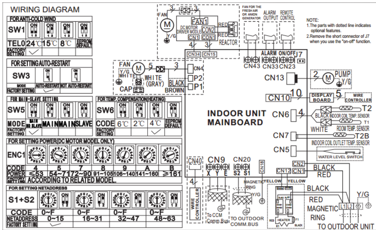
Fig. 21 — Wiring Diagram Sizes 36K- 48K
