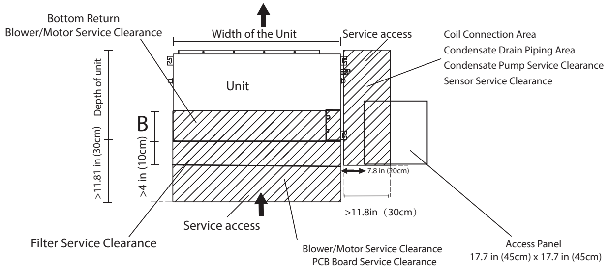
Fig. 6 — Maintenance Clearances
