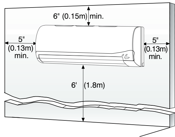
Fig. 2 – 40MVC Clearance
