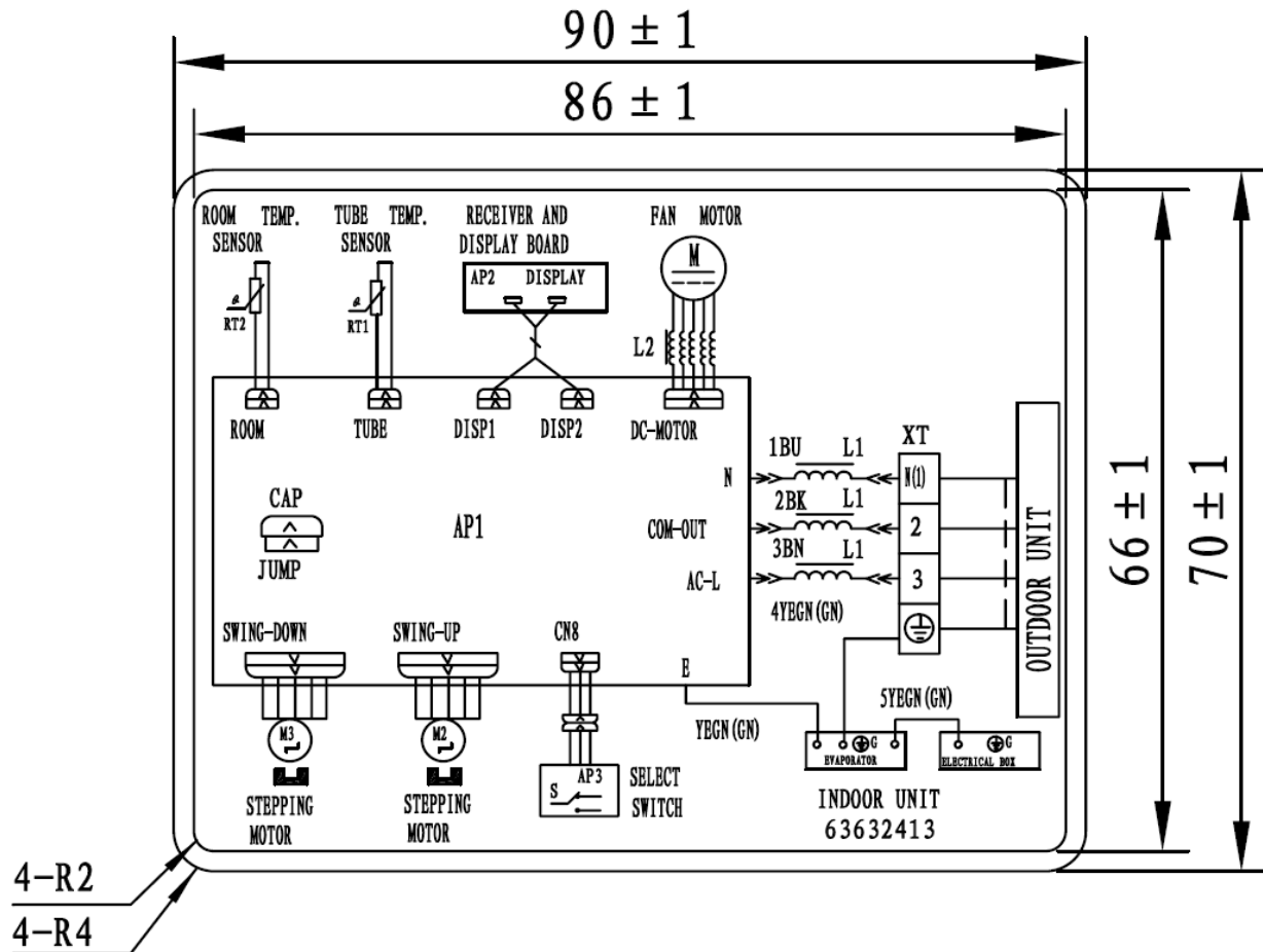
Fig. 20 – Wiring Diagrams GJ*F Floor Console 9k, 12k and 18k
