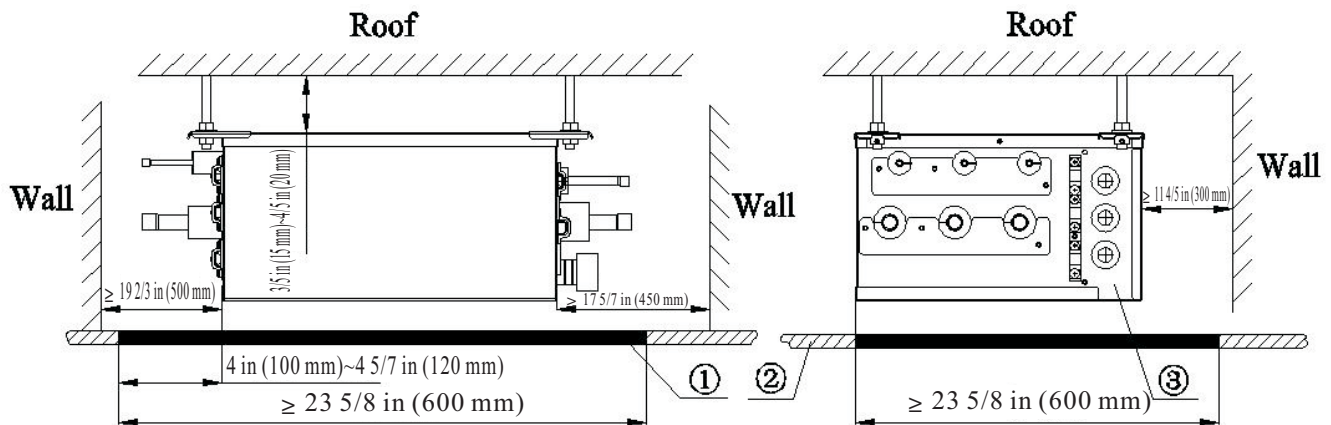
Fig. 17 – Installation and Service Space
