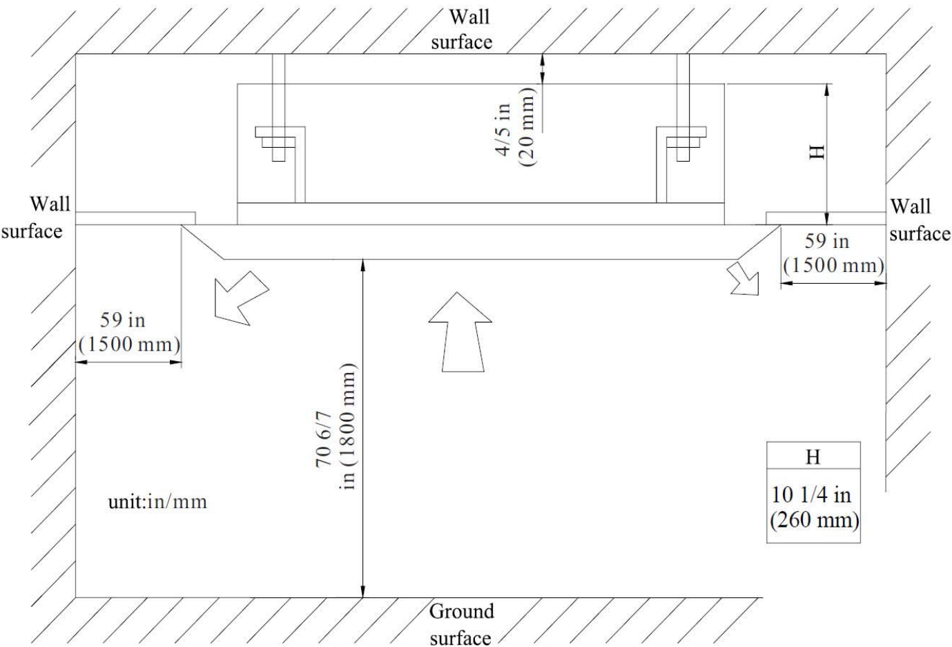
Fig. 19 – Cassette Clearance
