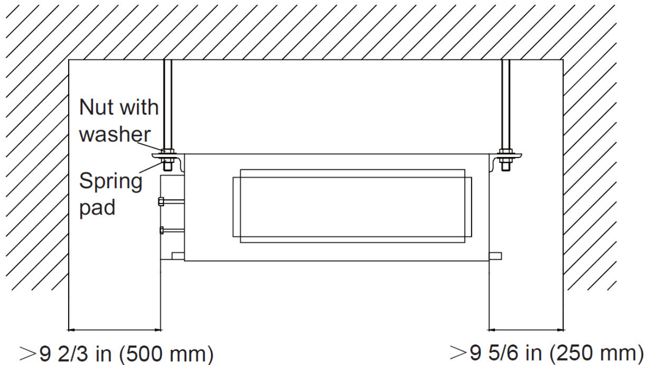
Fig. 20 – Ducted clearance
