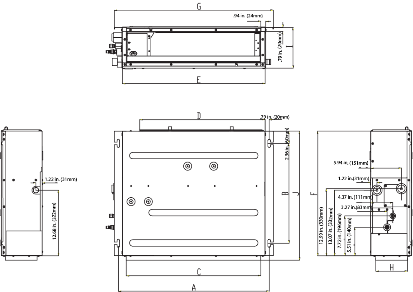
Fig. 8 – Ducted Dimensions
