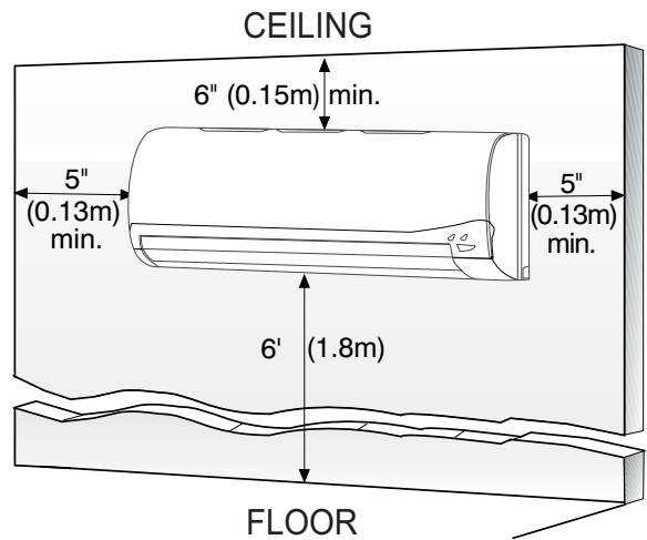
Fig. 18 – GR and GJ*B High Wall Clearance
