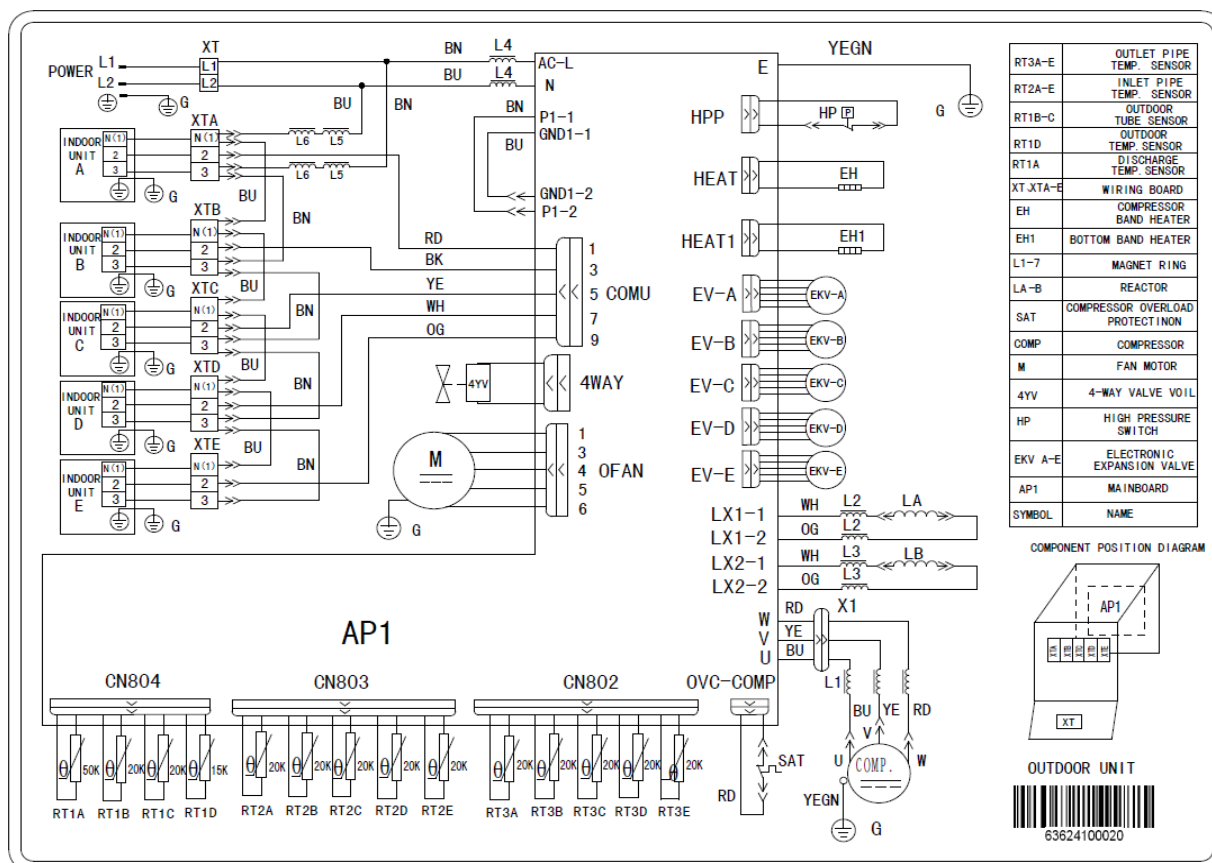
Fig. 29 – Wiring Diagram GJ Outdoor 36k and 42k
