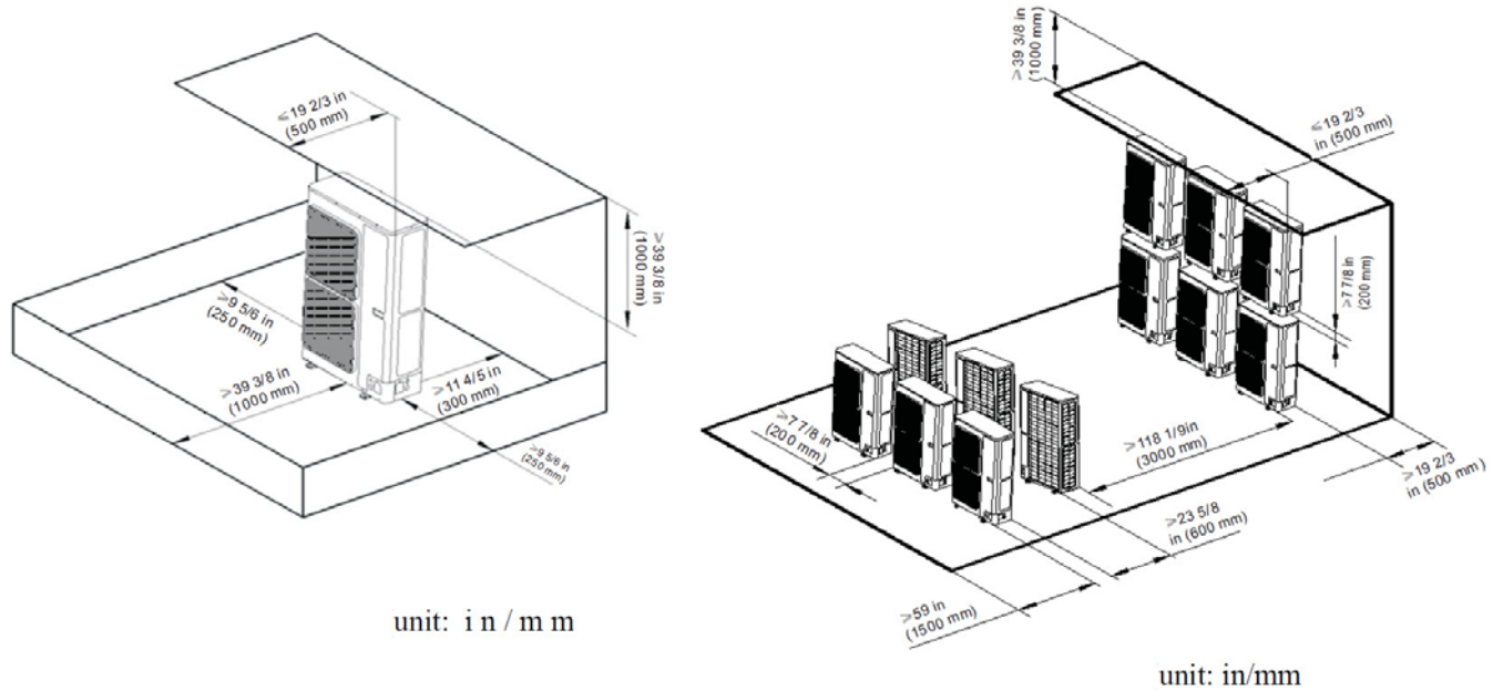
Fig. 23 – Clearances Outdoor 48-56
