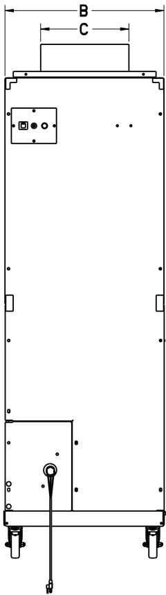
FRONT VIEW
