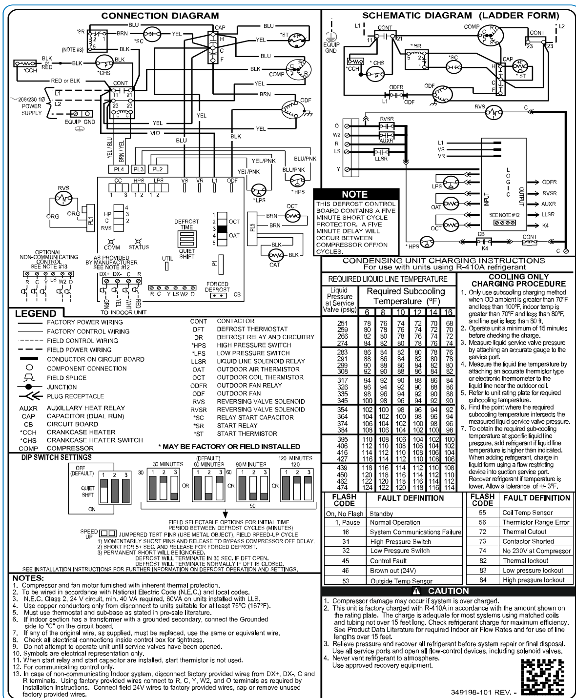
Fig. 1 – 18-60 Wiring Diagram
