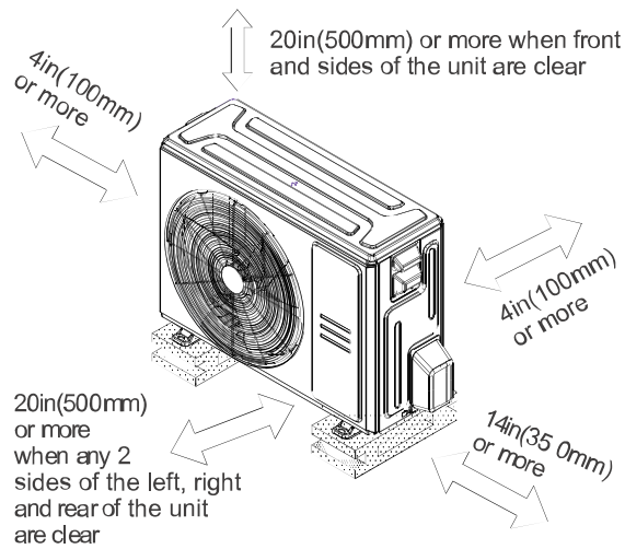
Fig. 5 – Clearances
