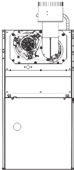
Fig. 4 - Chimney Adapter Secured to Upflow Furnace Flue Collar
