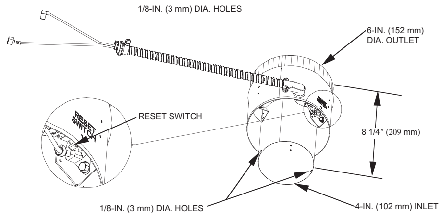
Fig. 14 - Chimney Adapters
