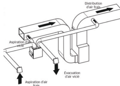
Fig. 9 – Installation Alternative
