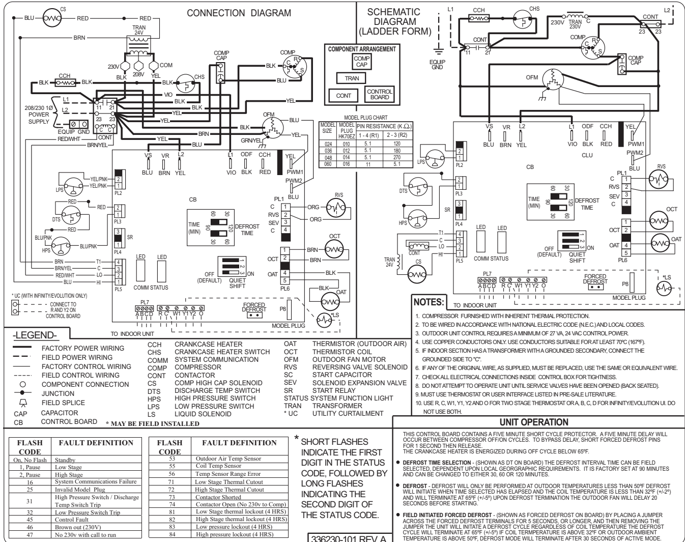
Fig. 1 – Wiring Diagram — Model size 2 - 5 tons, 208/230-1
