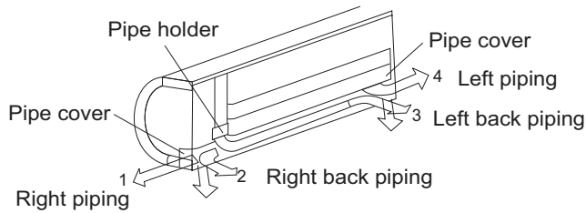
Fig. 4 — Piping Locations
