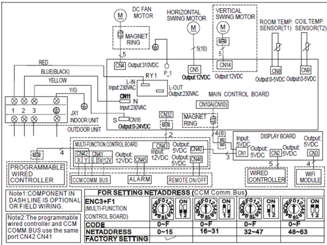
Fig. 8 — Wiring Diagram Sizes 18K - 24K (208/230V)
