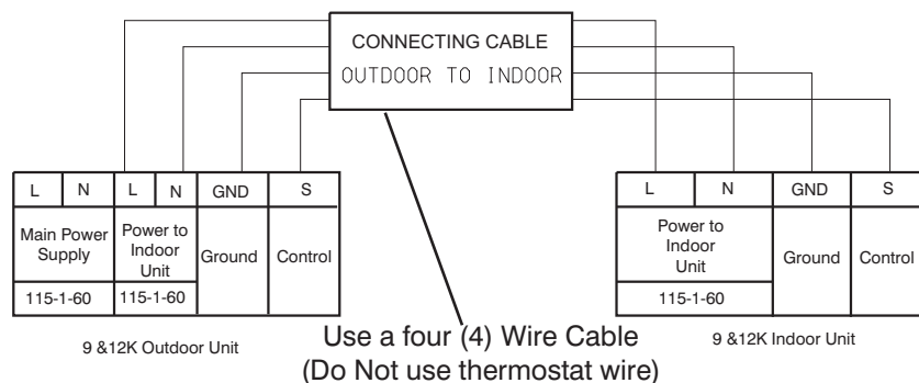
Fig. 7 – Connection Diagrams
