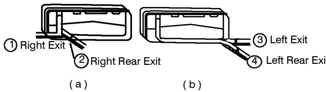
Fig. 11 – Refrigerant Line Routing
