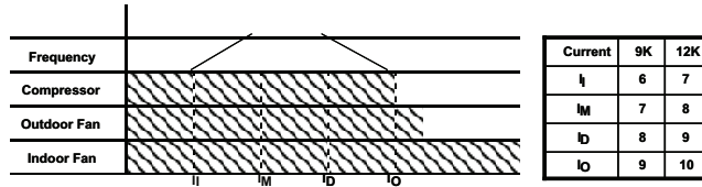
Fig. 17 – Overcurrent Protection
