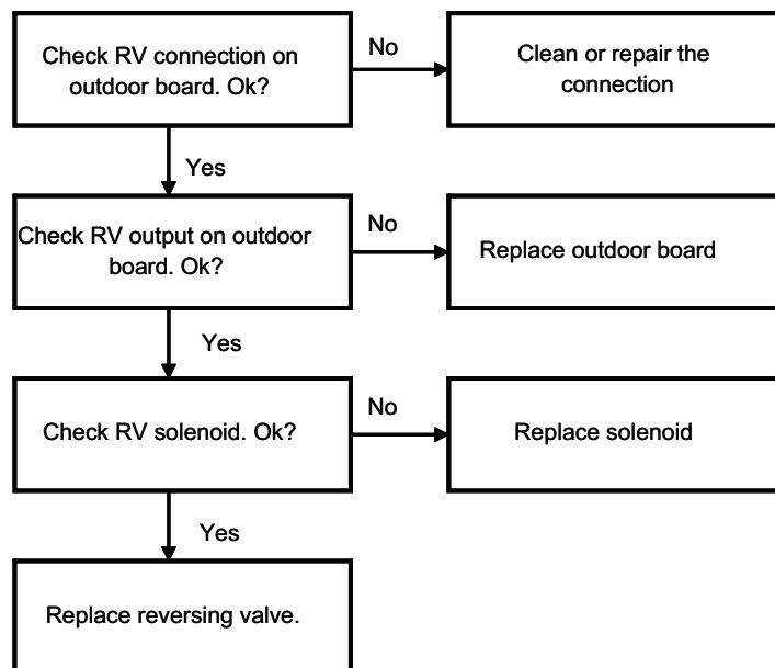
Fig. 39 – Reversing Valve
