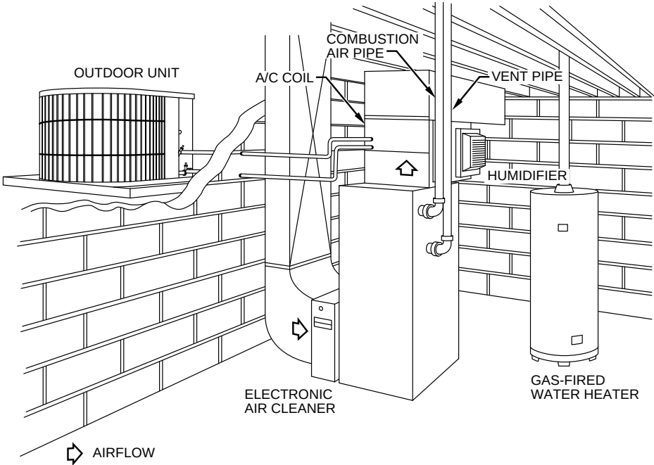
Basement — Upflow Application
