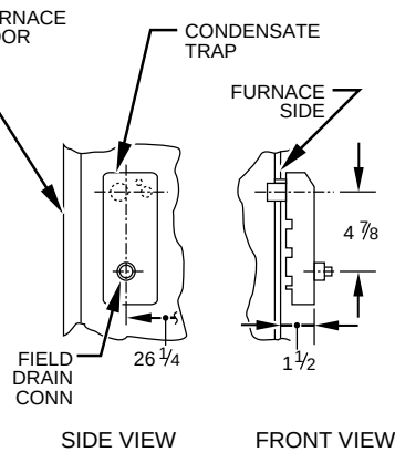
DOWNFLOW AND ALTERNATE EXTERNAL UPFLOW APPLICATIONS
