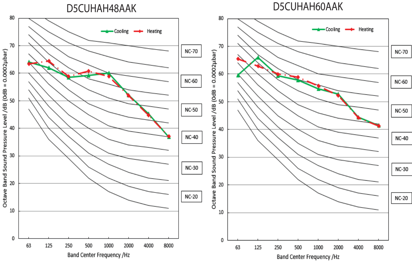
Fig. 17 —Sound Octave Bands
