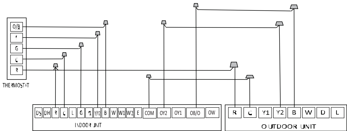
Fig. 33 —Wiring for 1H and 1C thermostat
