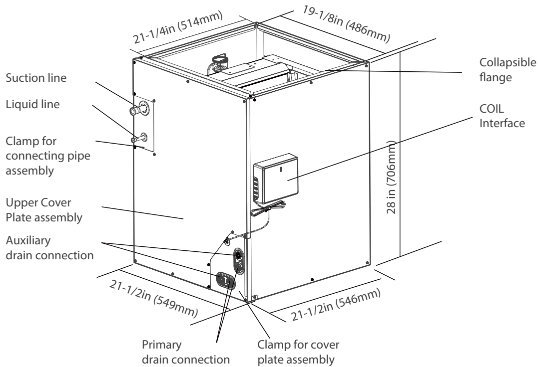
Fig. 3 – Model D5FULAH60XMX Dimensions
