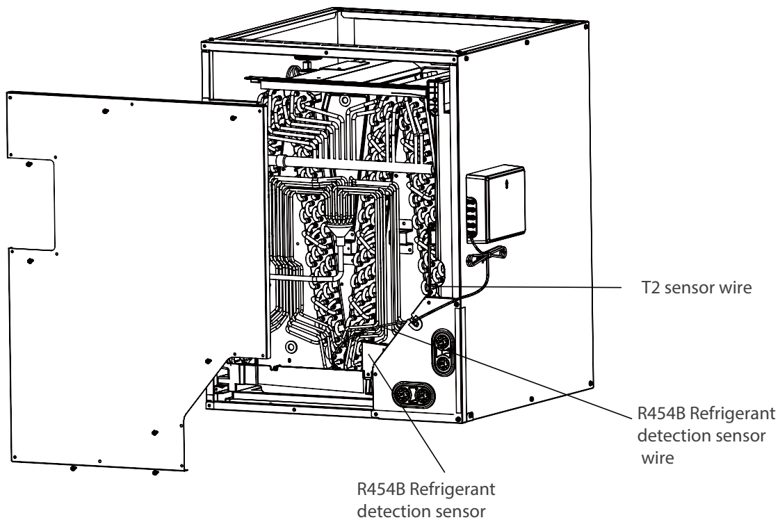
Fig. 4 – R-454B Sensor Location - Model D5FULAH60XMX
