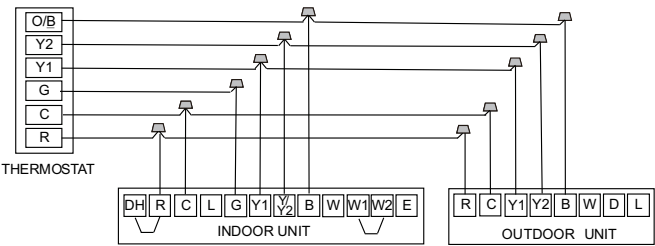
Fig. 11 —Wiring for 2H and 2C Thermostat
