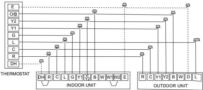
Fig. 9 —Wiring for 3H and 2C Thermostat
