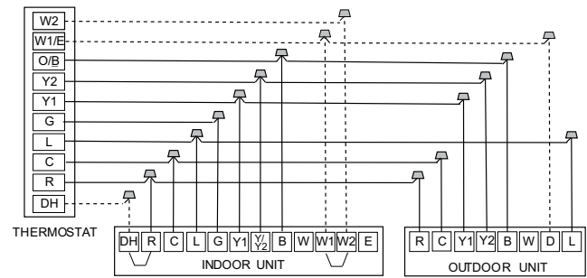
Fig. 7 —Wiring for 4H and 2C Thermostat
