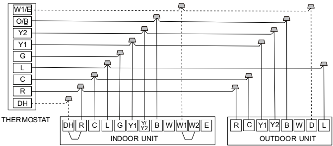
Fig. 10 —Wiring for 3H and 2C Thermostat
