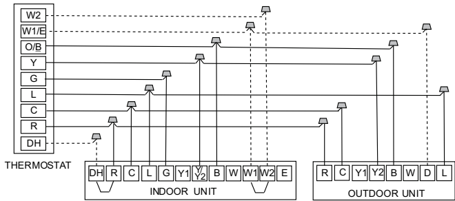
Fig. 8 —Wiring for 3H and 1C Thermostat
