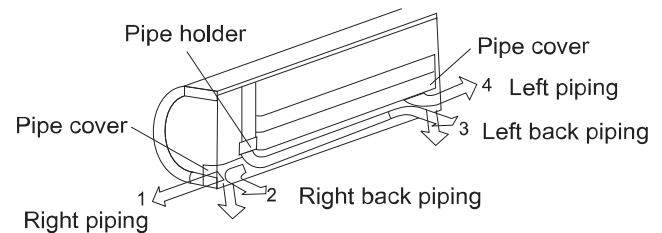
Fig. 10 — Piping Connections
