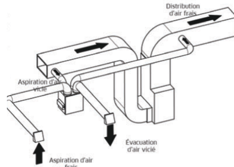
Fig. 9 – Installation Alternative
