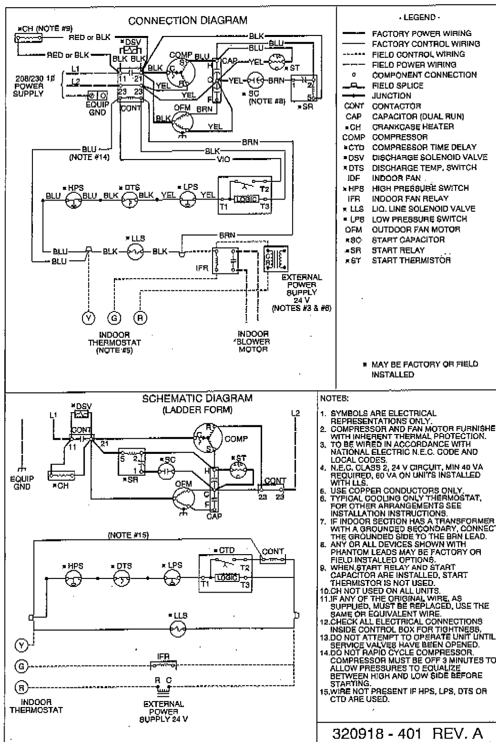
Fig. 1—597C024-048 208/230v, 1 Phase, 60 Hertz
