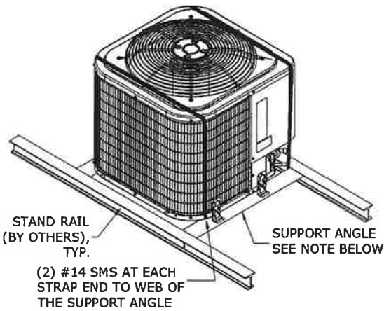
3 MECHANICAL UNIT N.T.S. FRONT ISOMETRIC
