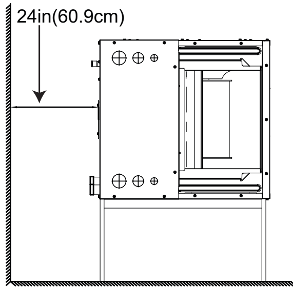
Horizontal Installations
