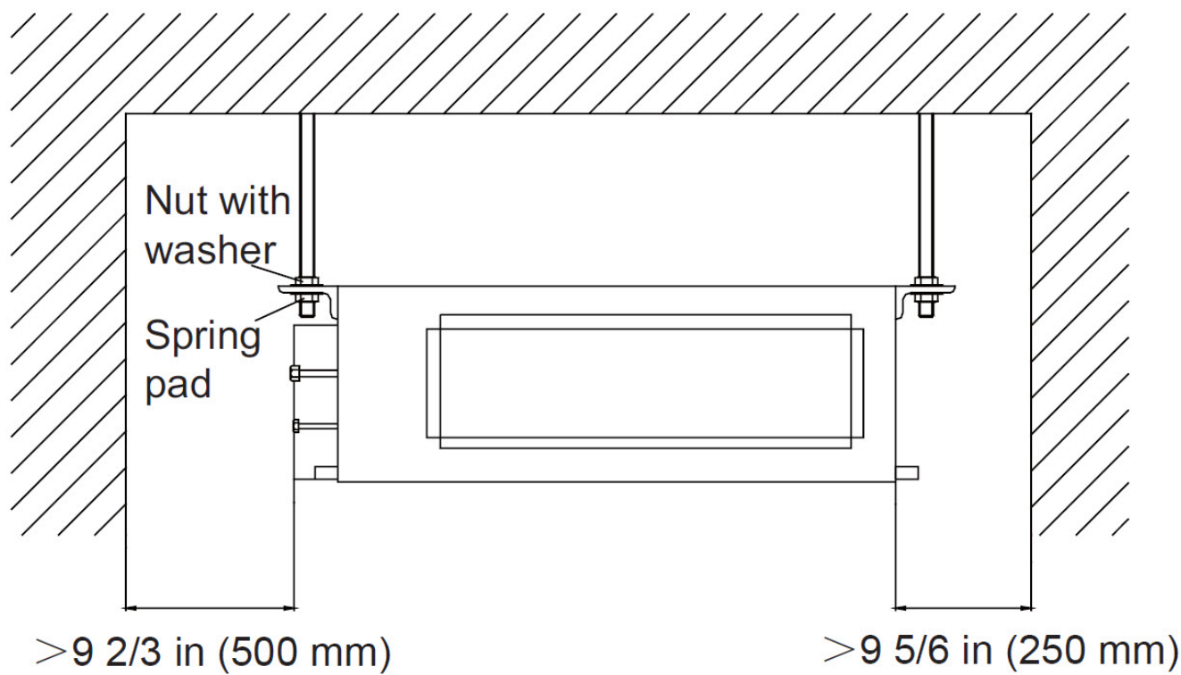
Fig. 26 – Ducted clearance
