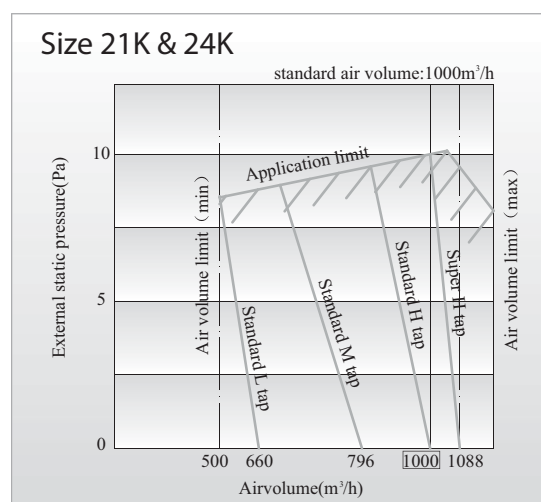
Fig. 24 – Fan Performances – SI Units of Measurement
