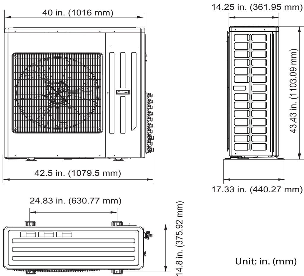
Fig. 11 – Outdoor Dimensions Size 36-42
