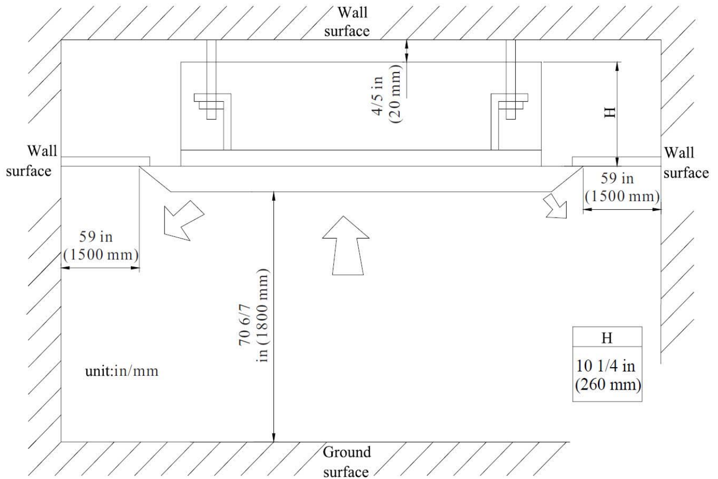
Fig. 25 – Cassette Clearance
