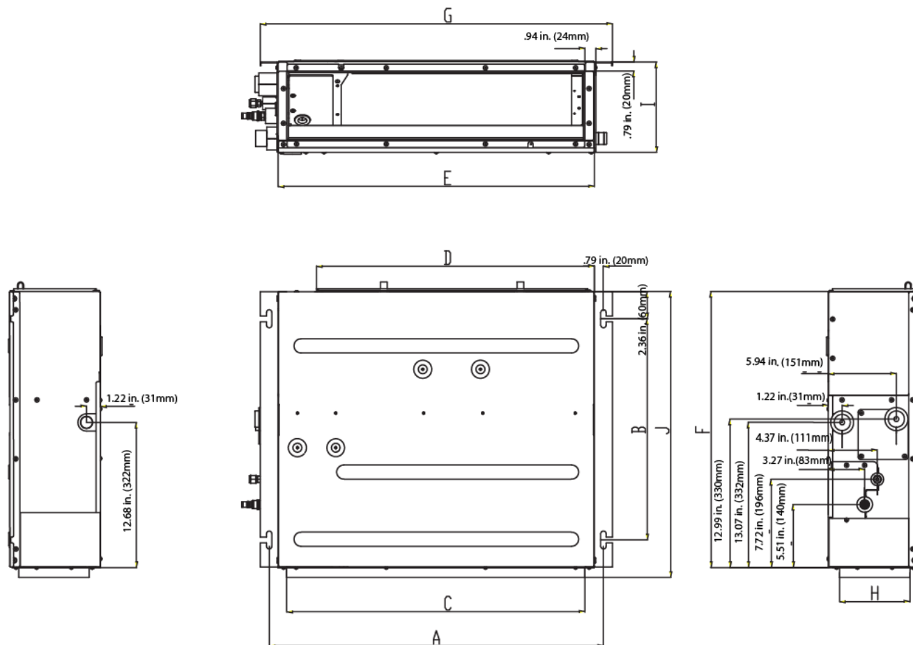
Fig. 6 – Ducted Dimensions
