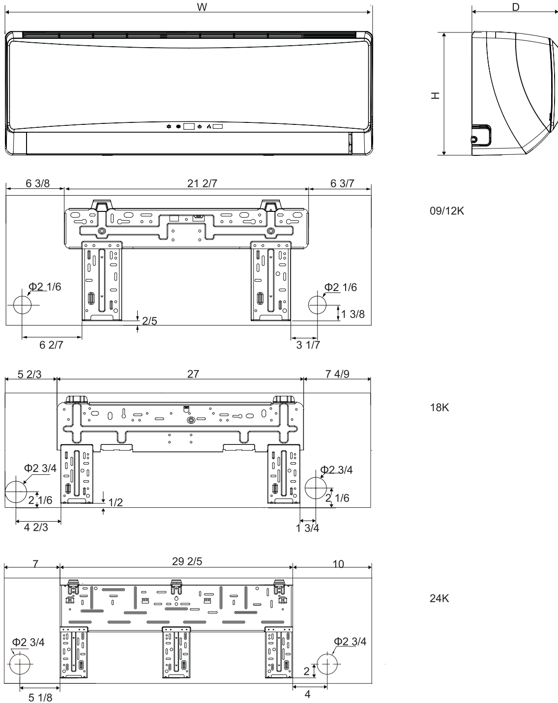
Fig. 3 – 40GJ*B High Wall Dimensions
