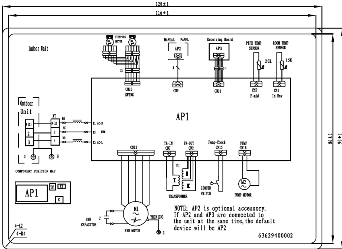
Fig. 30 – Wiring Diagram Cassette 12k, 18k
