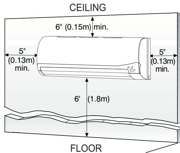
Fig. 24 – High Wall Clearance
