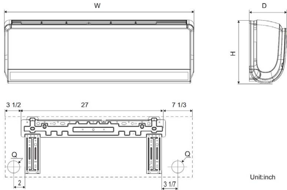
Fig. 2 – 40GR High Wall Dimensions
