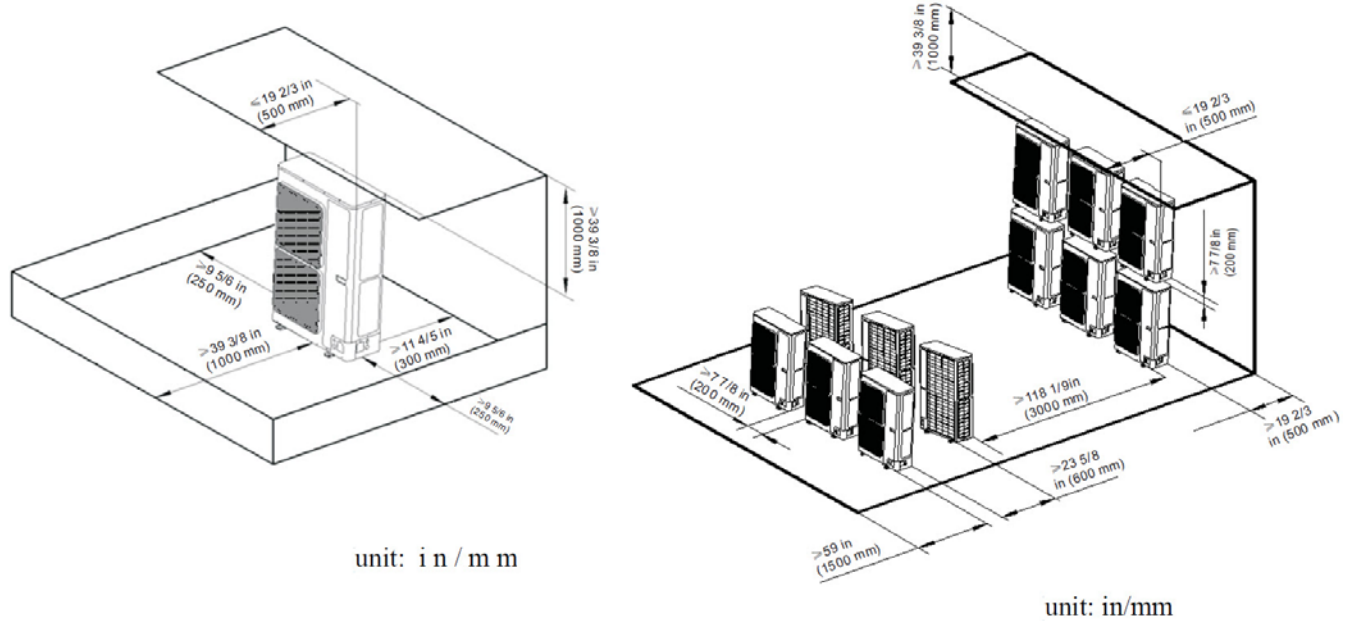
Fig. 29 – Clearances Outdoor 48–56
