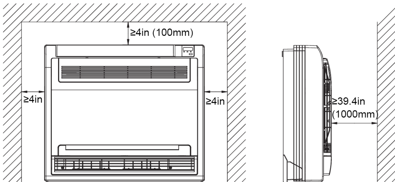
Fig. 27 – Floor Console clearance
