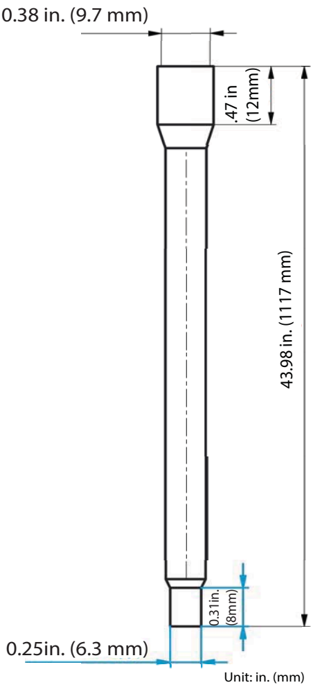
Fig. 21 – Piping Adapter Indoor Side (Liquid)
