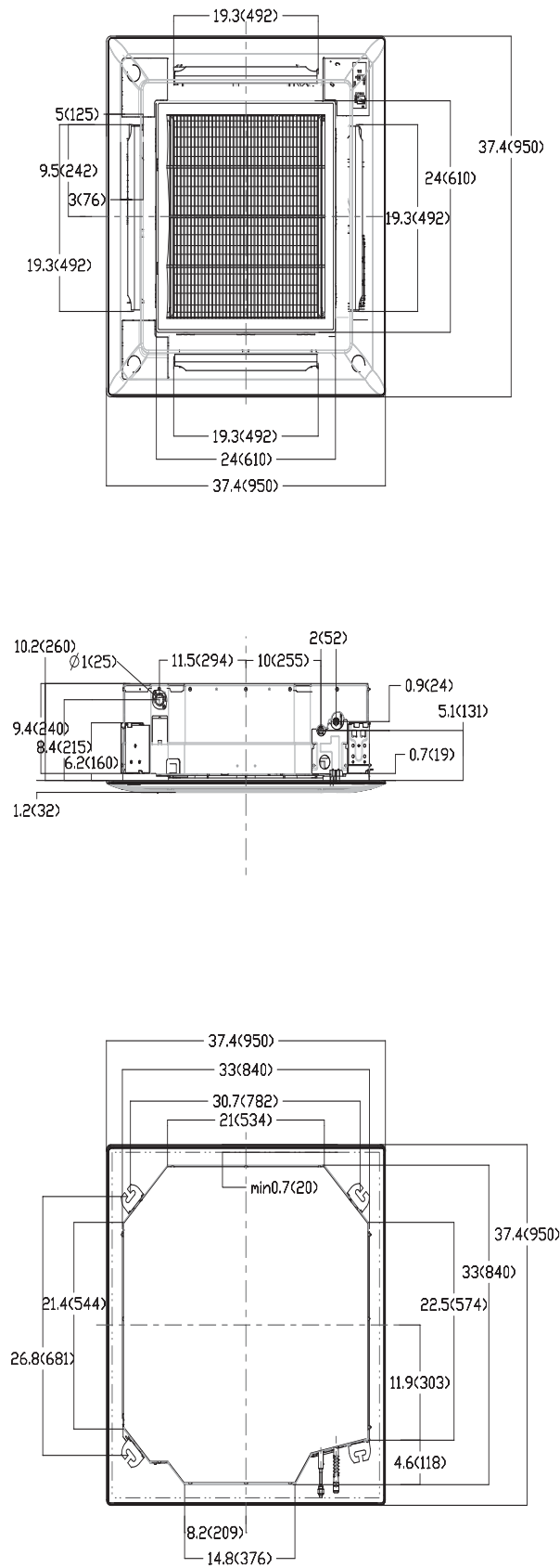
Fig. 5 – Cassette Dimensions Size 24
