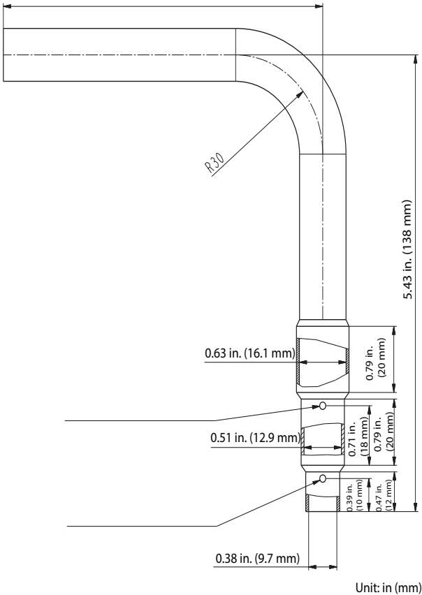
Fig. 19 – Piping Adapter Indoor Side (Gas)
