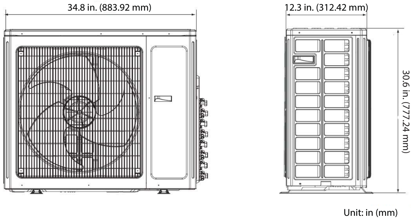
Fig. 9 – Outdoor Dimensions Size 24
