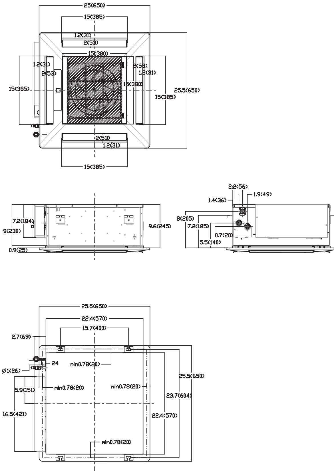
Fig. 4 – Cassette Dimensions Size 12 and 18
