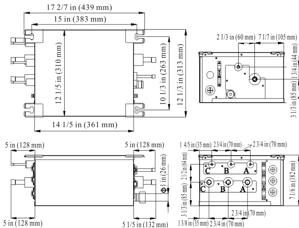
Fig. 15 – Outline Dimensions
