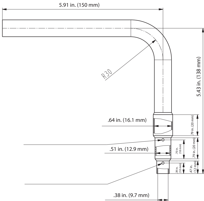
Fig. 18 – Piping Adapter Indoor Side
