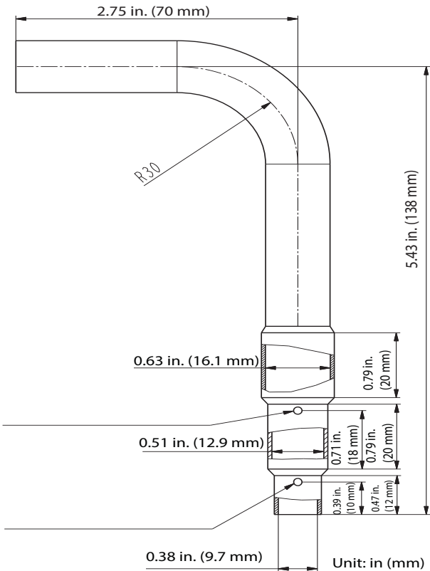
Fig. 20 – Piping Adapter Indoor Side (included only with KSAUI0401AAA)
