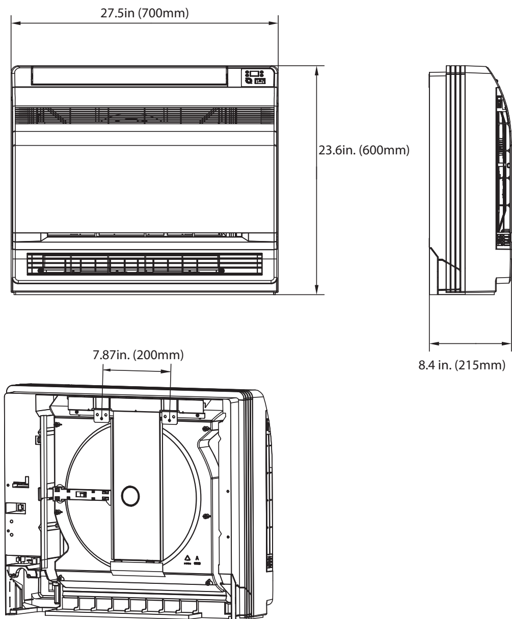
Fig. 7 – Floor Console Dimensions
