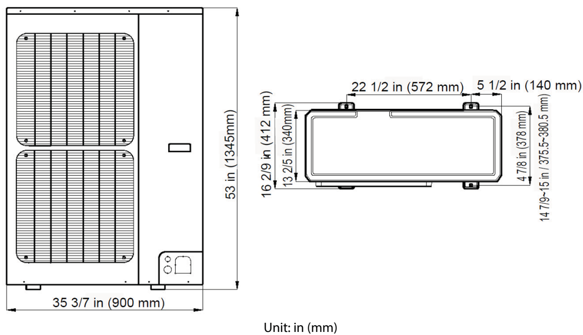
Fig. 12 – Outdoor Dimensions Size 48-56
