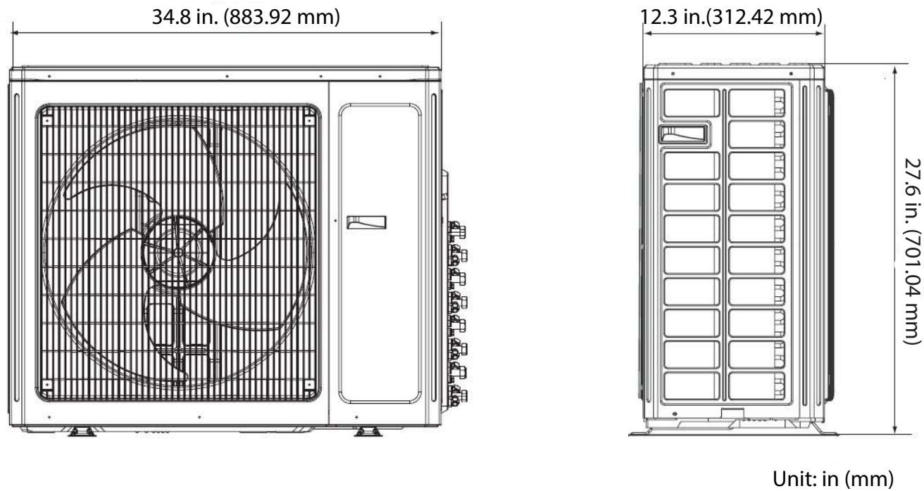
Fig. 8 – Outdoor Dimensions Size 18
