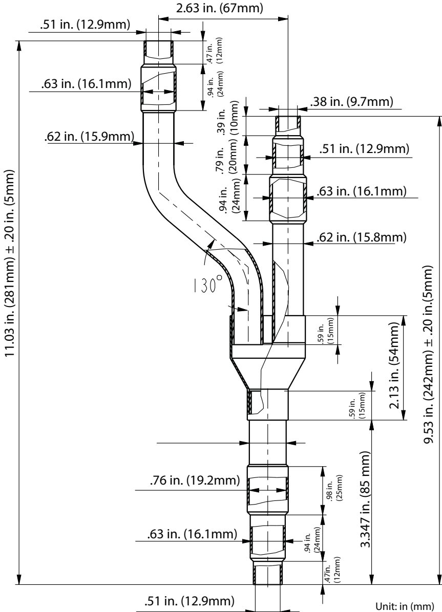
Fig. 22 – Branch Pipe – Gas Pipe
