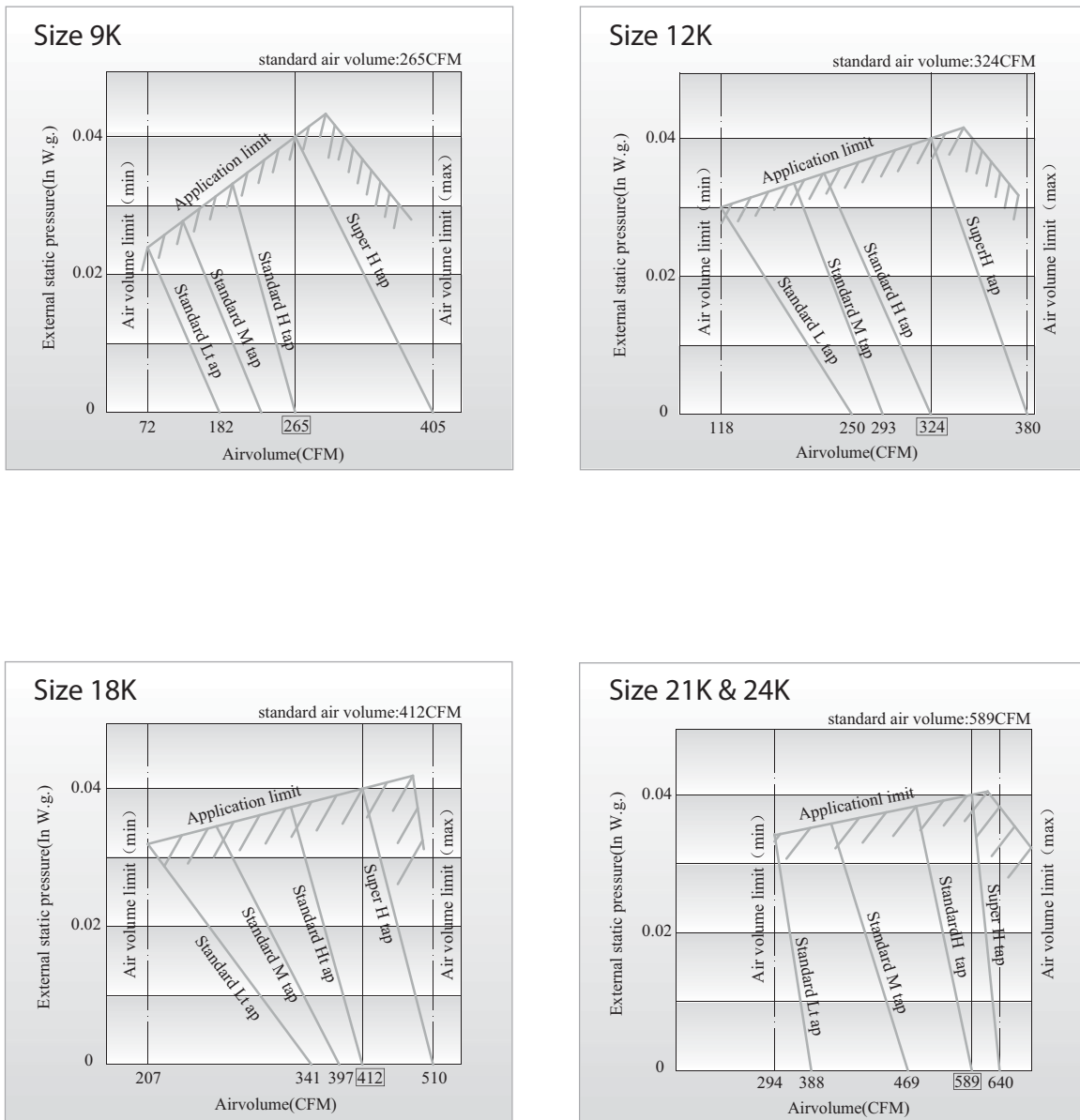
Fig. 25 – Fan Performances – US Units of Measurement
