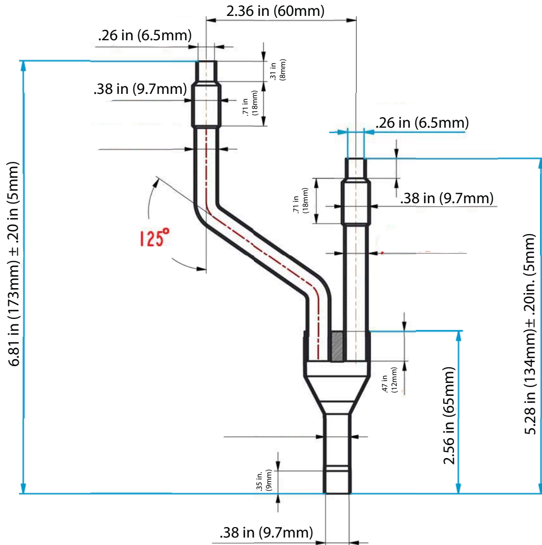
Fig. 23 – Branch Pipe – Liquid Pipe
