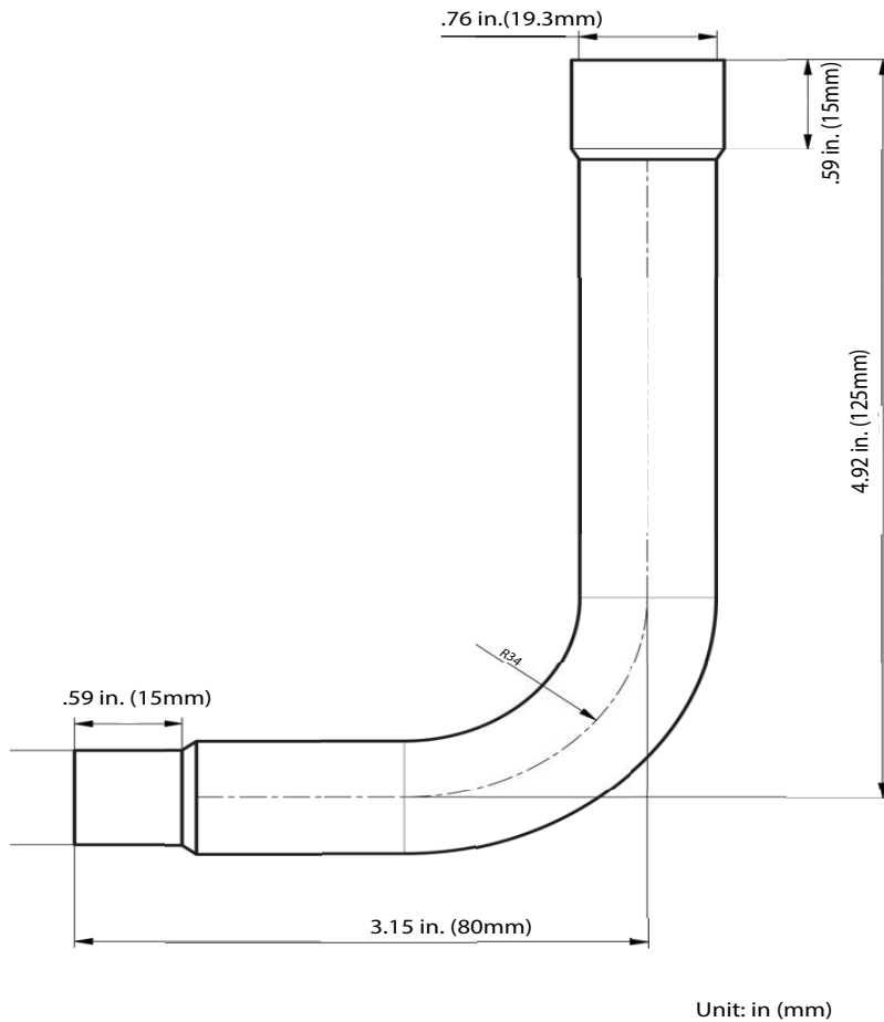
Fig. 17 – Piping Adapter Outdoor
