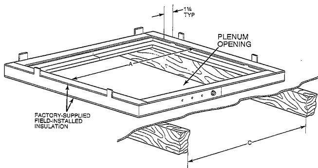
Assembled
