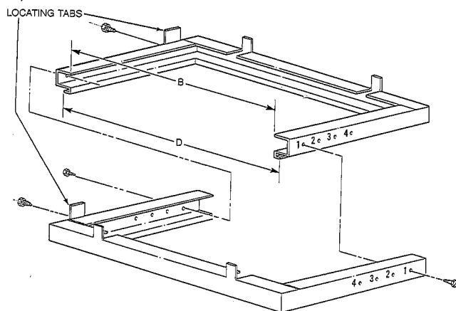
Disassembled
