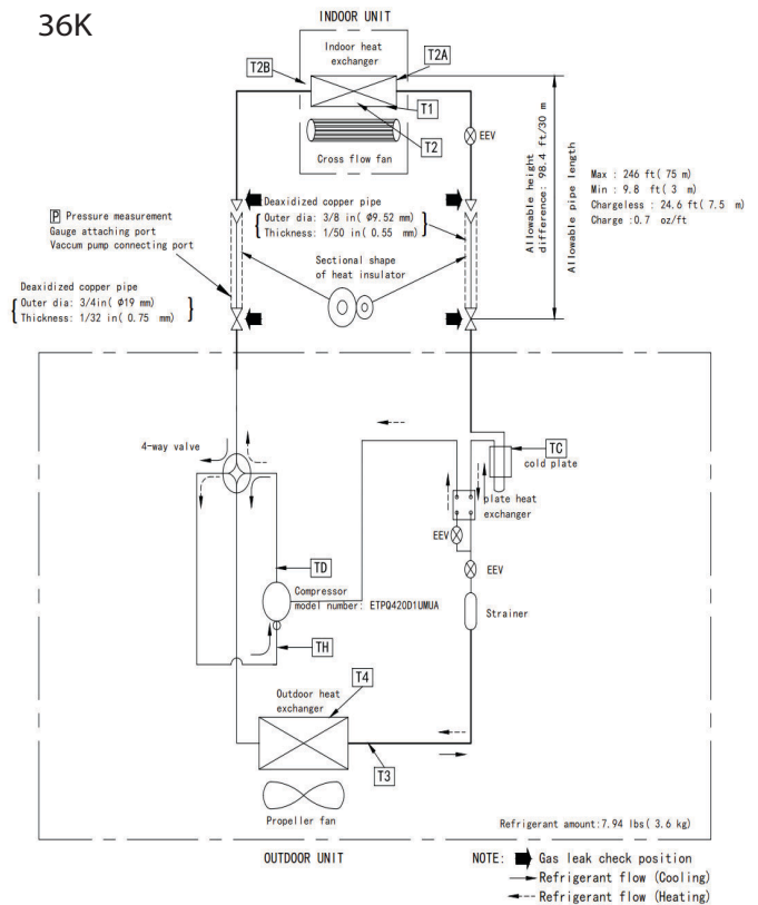
Fig. 24 —Refrigerant Cycle 30K, 36K
