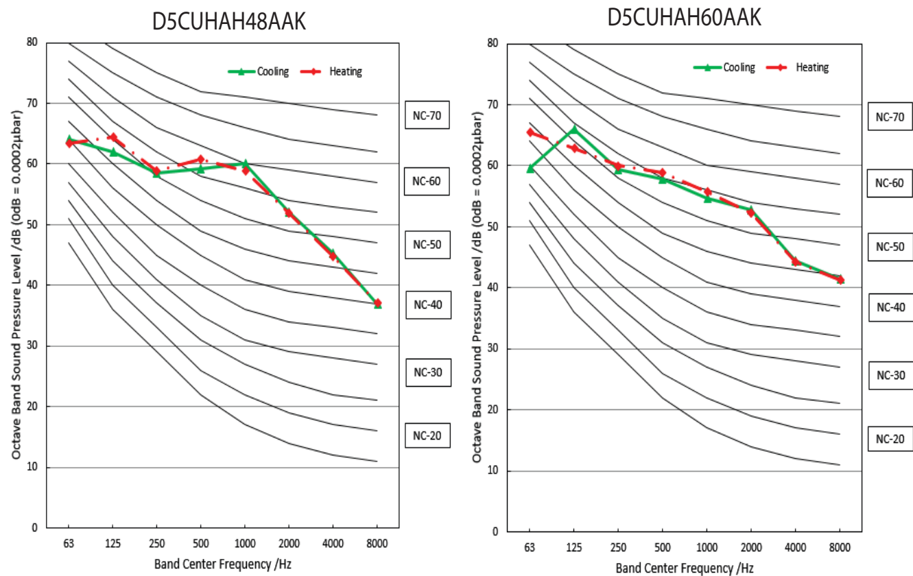
Fig. 16 —Sound Octave Bands
