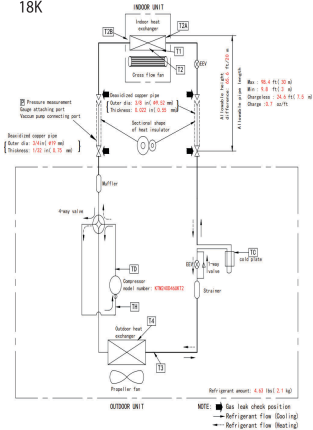
Fig. 23 —Refrigerant Cycle 18K, 24K
