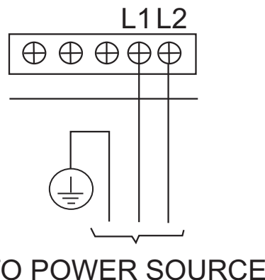
Fig. 10 — Match Fork Terminal to Terminal Labels
