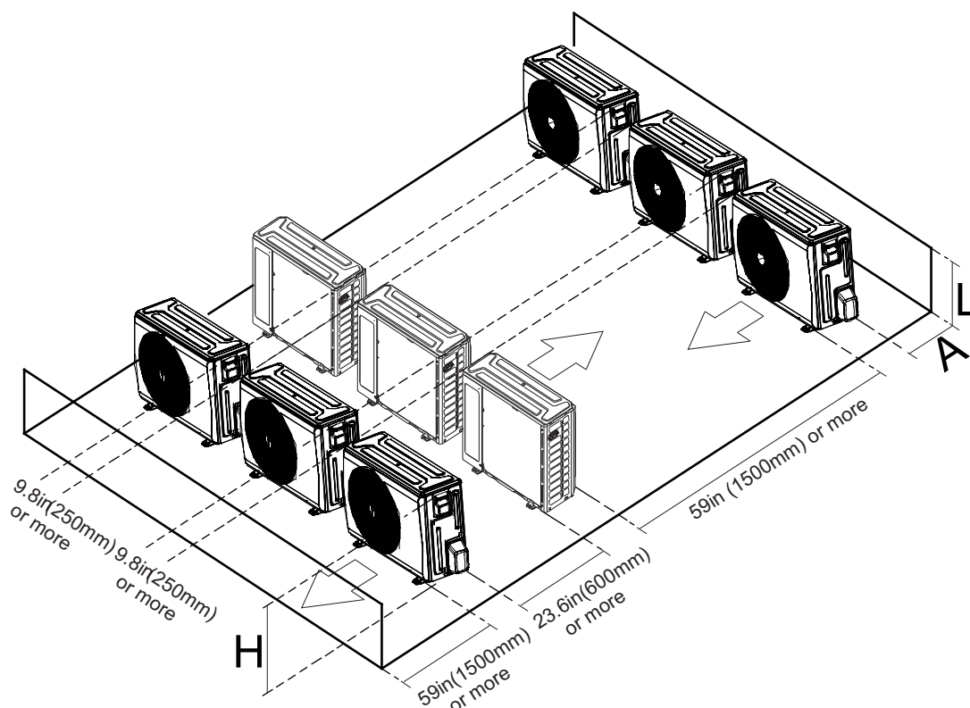
Fig. 8 – Clearance for Multiple Units
