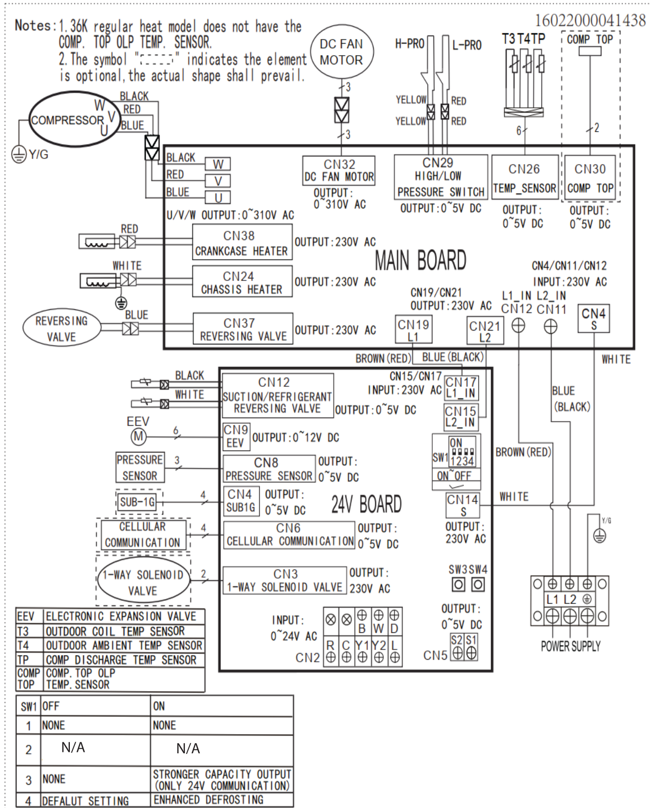
Fig. 27 — Wiring Diagram Size 30K
