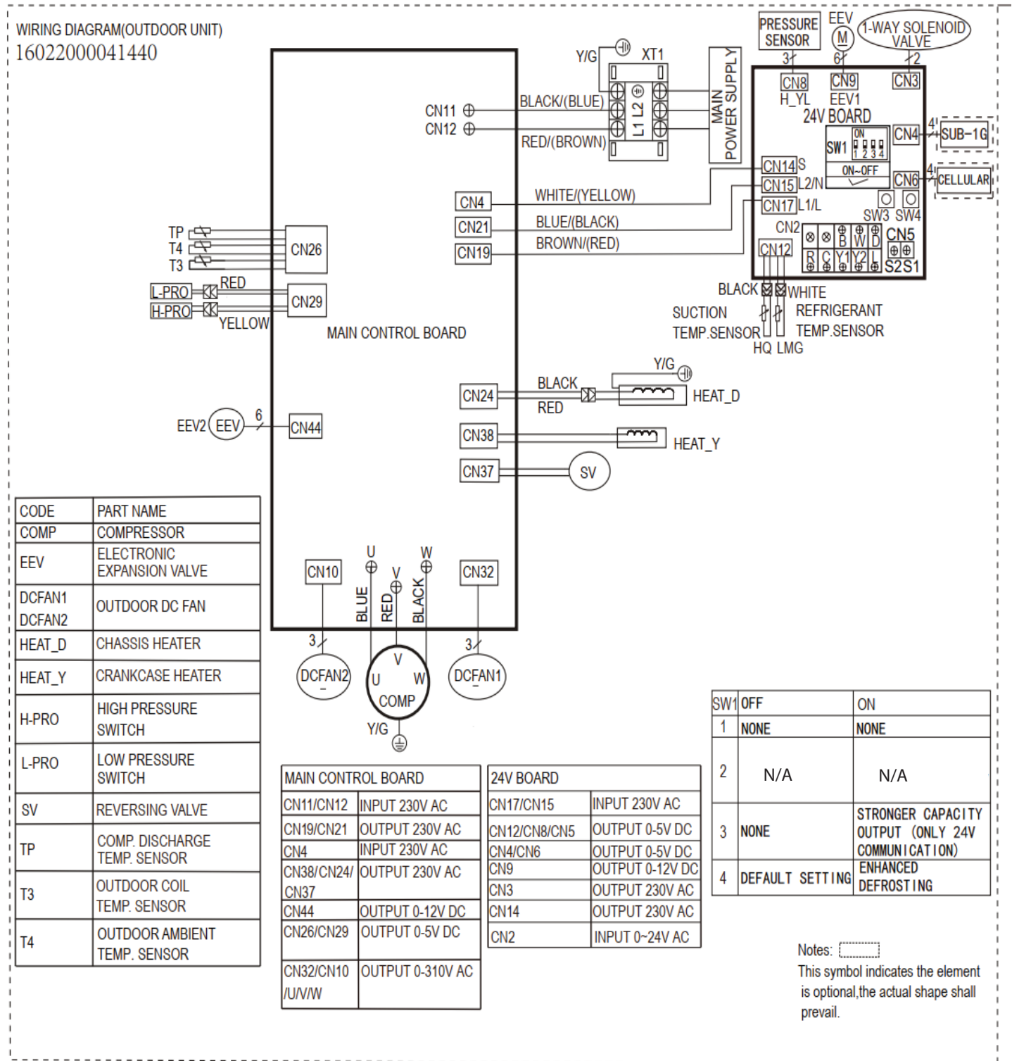
Fig. 29 — Wiring Diagram Size - 60K
