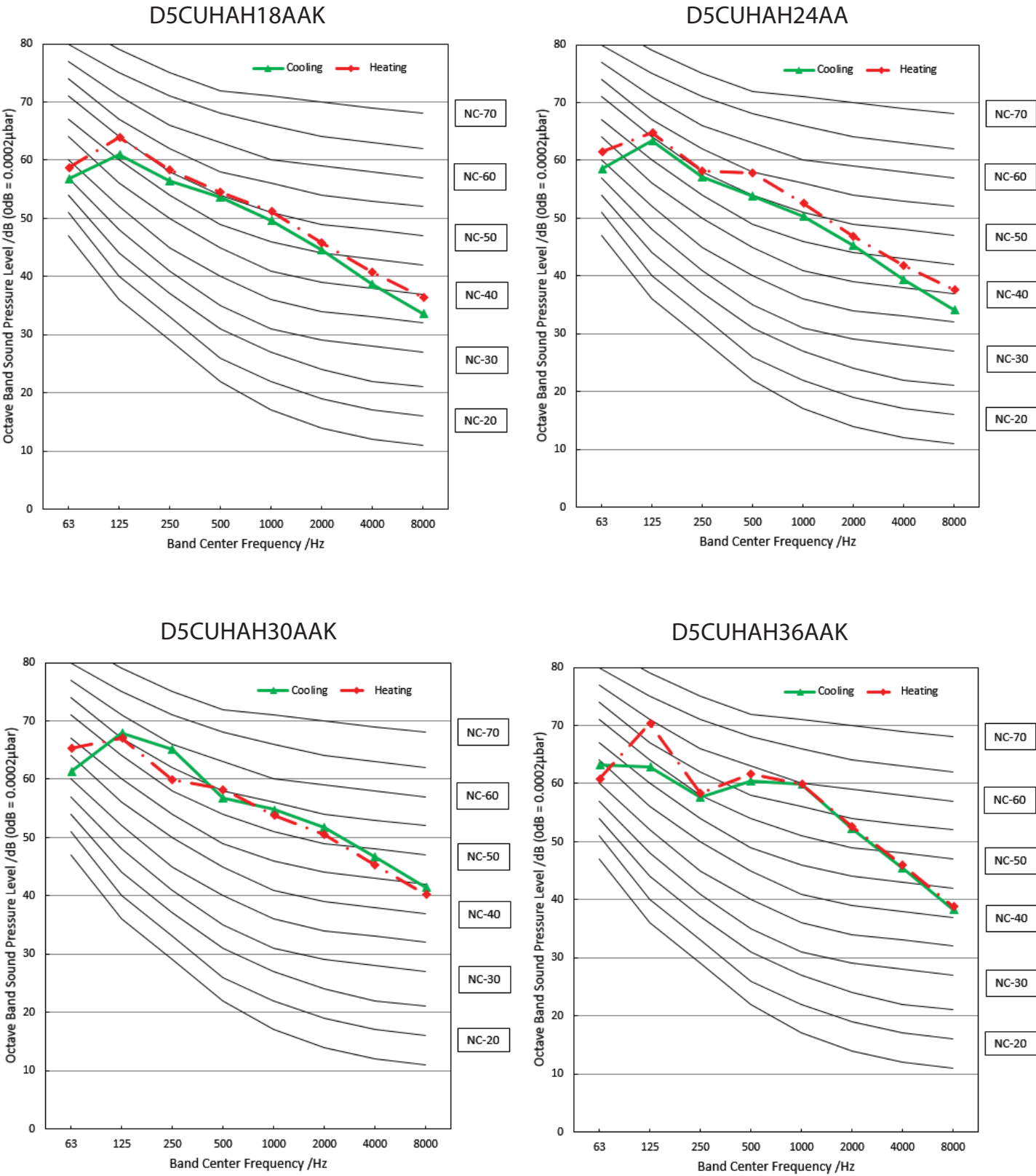
Fig. 15 — Sound Octave Bands
