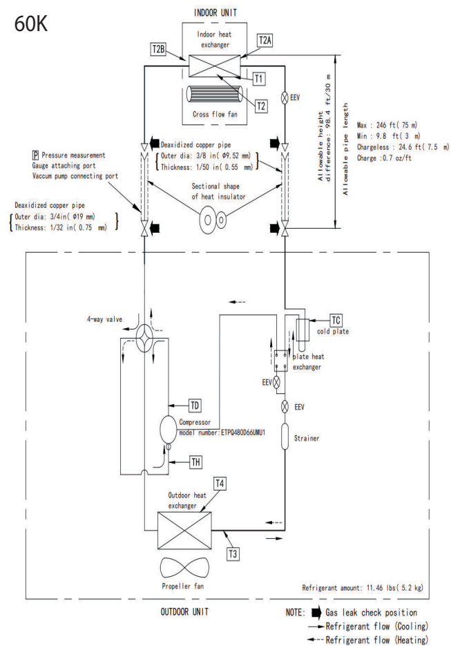
Fig. 25 — Refrigerant Cycle 48K, 60K
