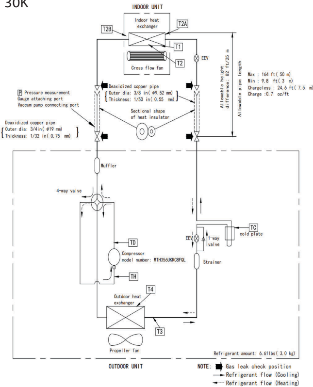
Fig. 24 —Refrigerant Cycle 30K, 36K
