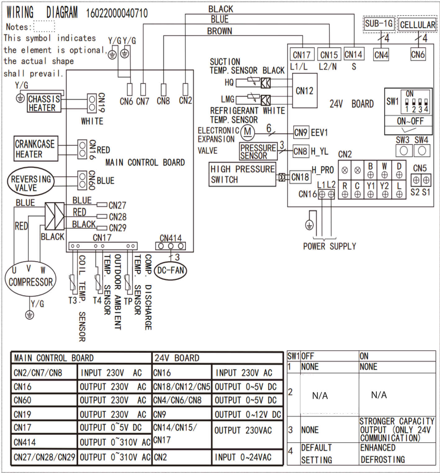
Fig. 26 — Wiring Diagram Sizes18K and 24K
