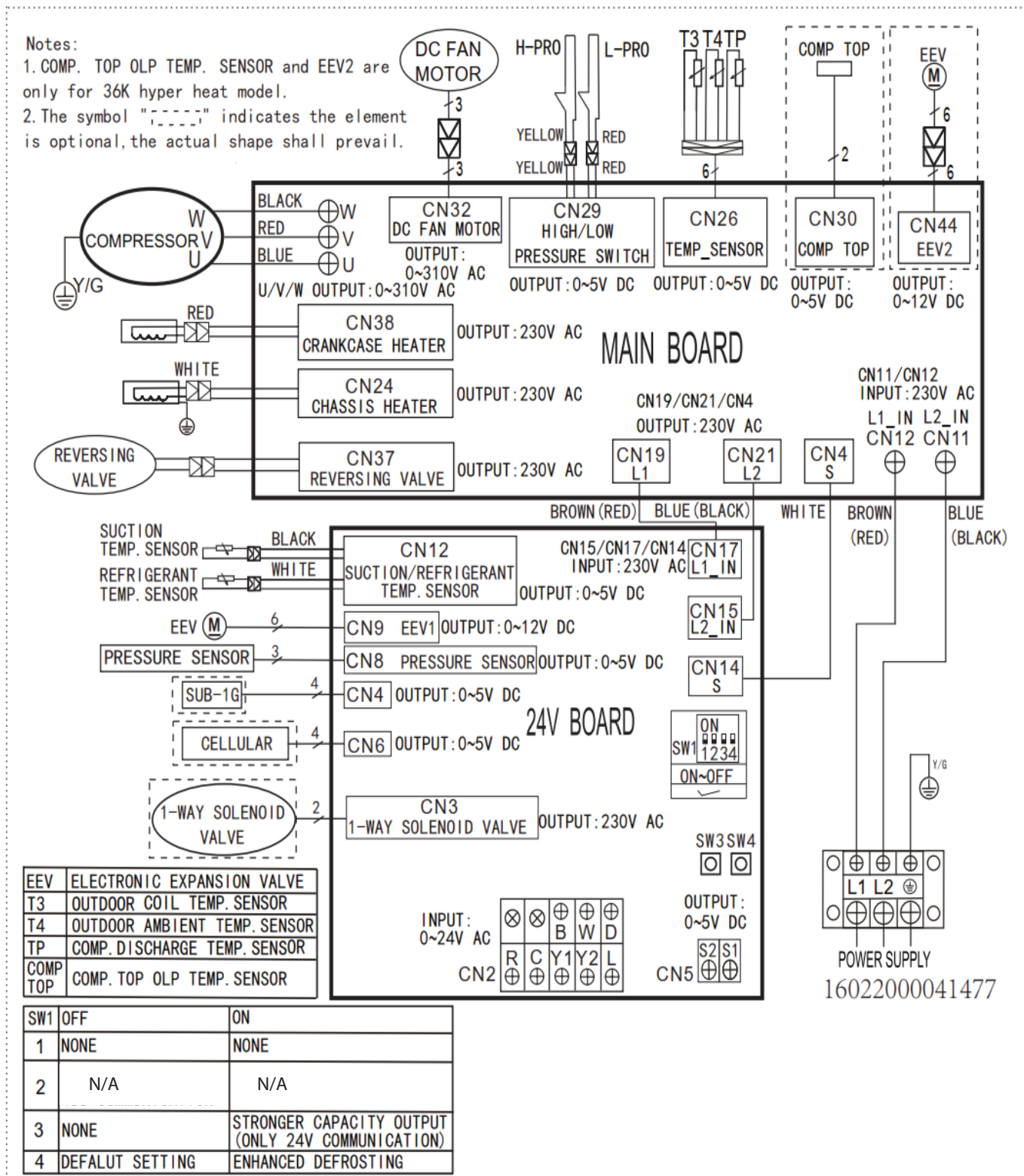
Fig. 28 — Wiring Diagram Sizes 36K - 48K
