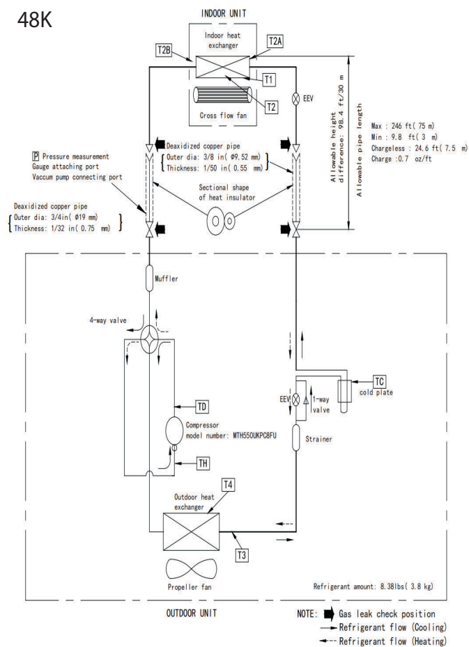
Fig. 25 — Refrigerant Cycle 48K, 60K
