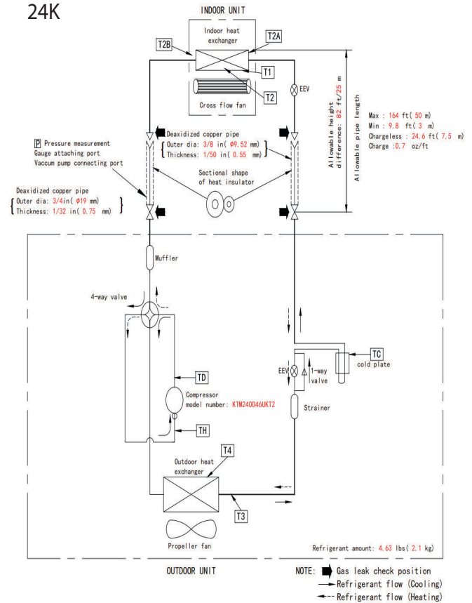
Fig. 23 —Refrigerant Cycle 18K, 24K
