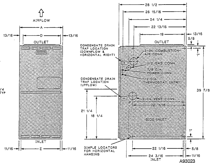
DIMENSIONS (IN.)
