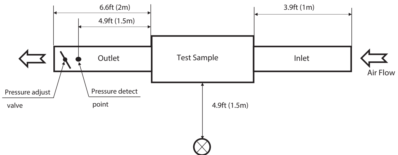
Fig. 7 — Sound Pressure Testing Method
