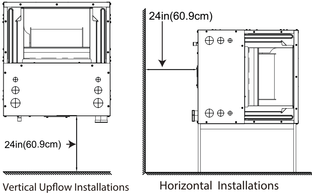
Fig. 4 — Clearances
