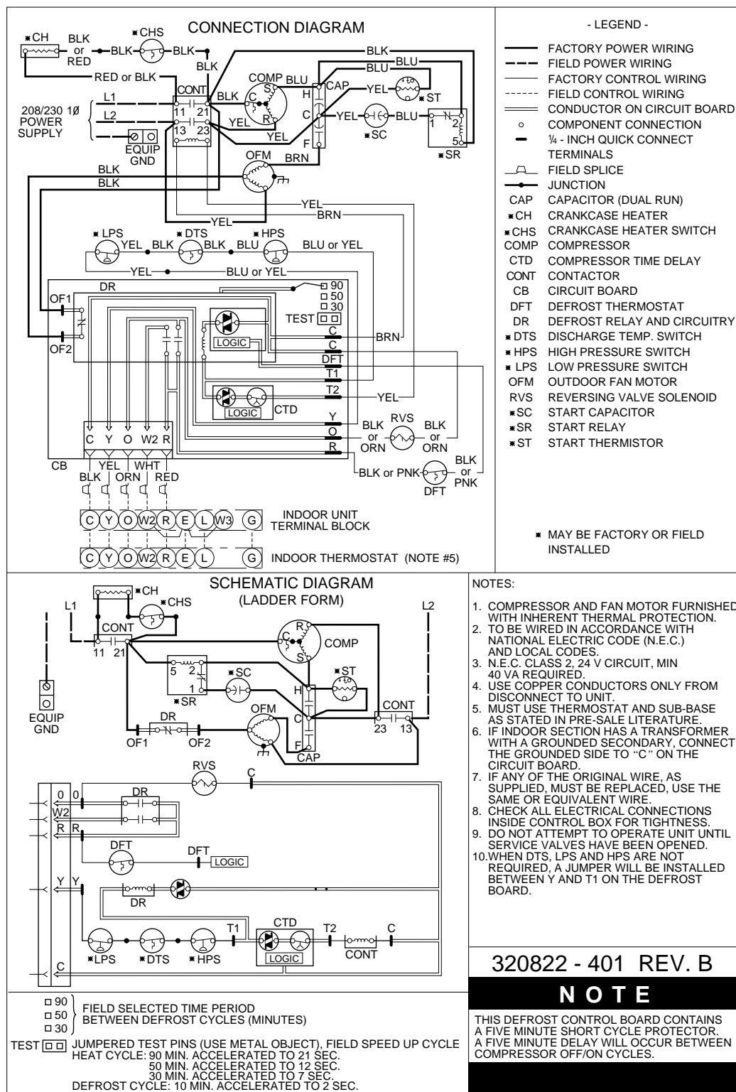
Fig. 2—38BY060 208/230v, 1 Phase, 60 Hertz
