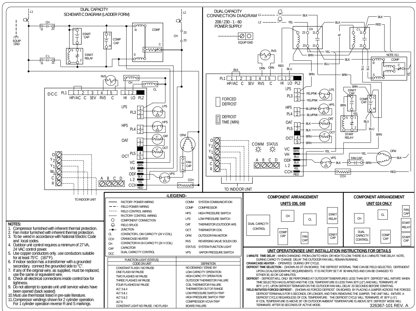
Fig. 1—Wiring Diagram—024, 036, 048
