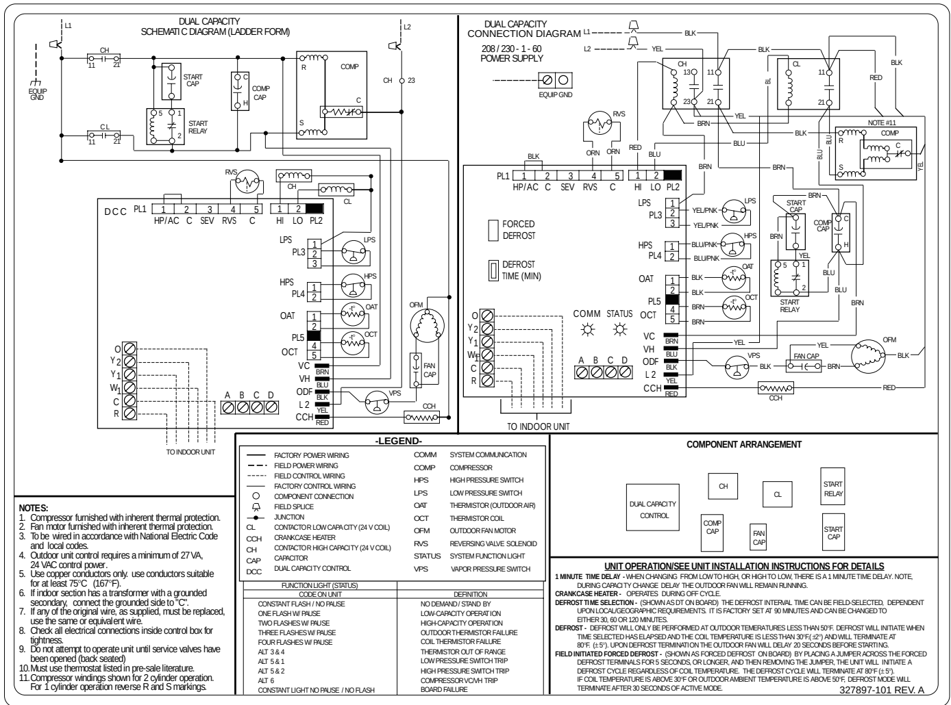
Fig. 3—Wiring Diagram—060
