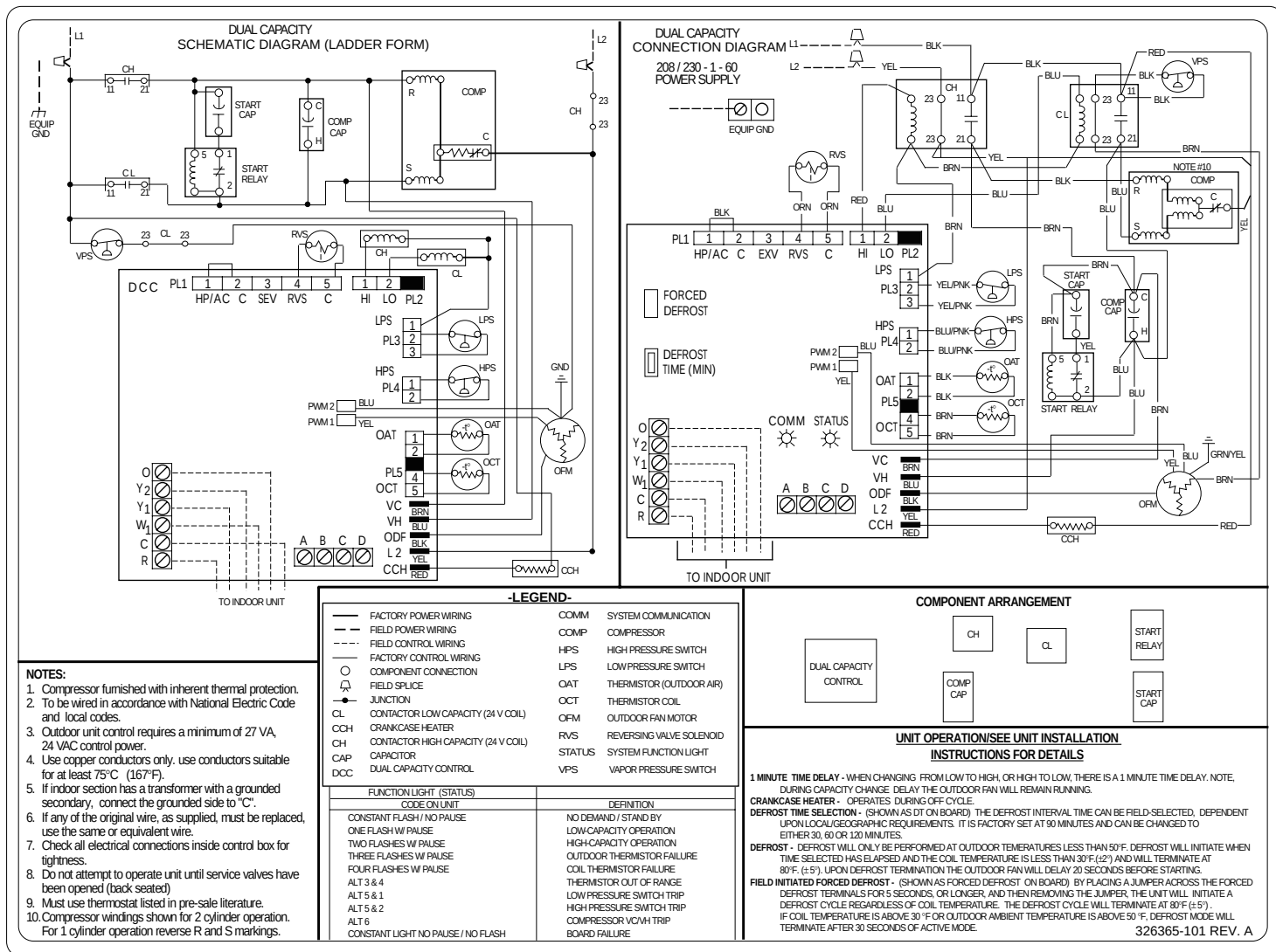
Fig. 2—Wiring Diagram—037
