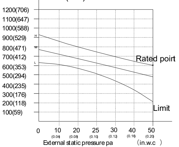
Air volume m3/h(CFM)
