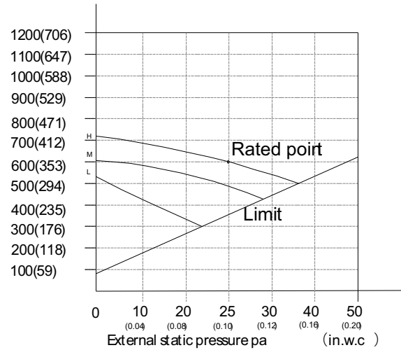
Air volume m3/h(CFM) SP2
