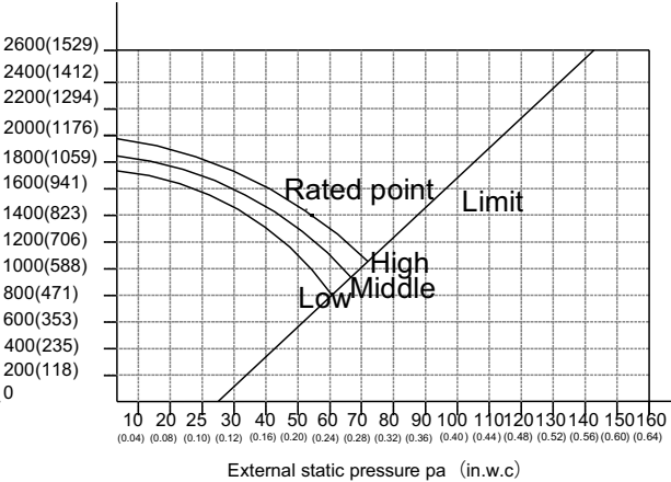
Air volume m3h(CFM) SP2
