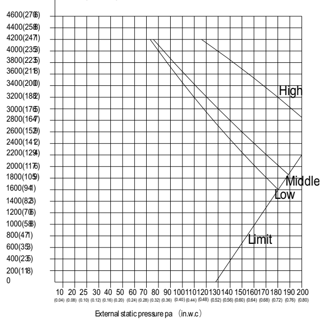
Air volume m 3 /h(CFM) SP4
