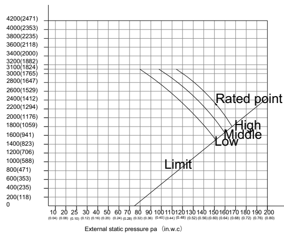
Air volume m3h(CFM) SP3
