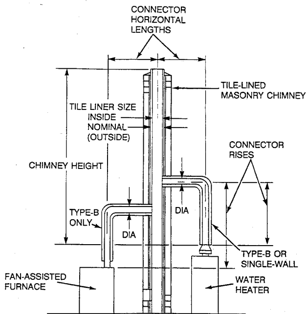
Fig. 3—Use With Tables 5, 6, 14 and 15 A91202
