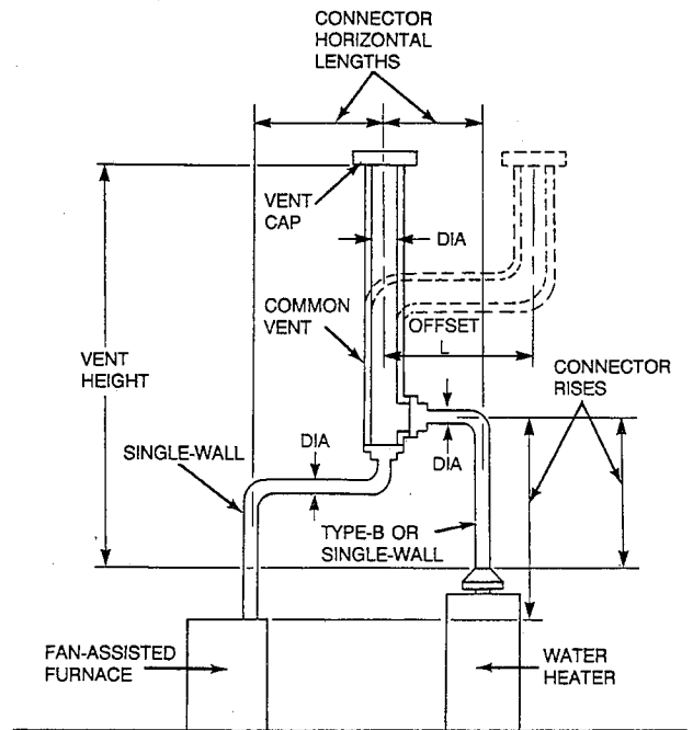
Fig. 2—Use With Tables 3 and 4 A91201
