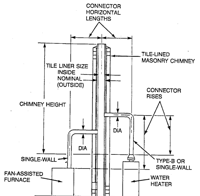
Fig. 4—Use With Tables 7 and 8 A91203
