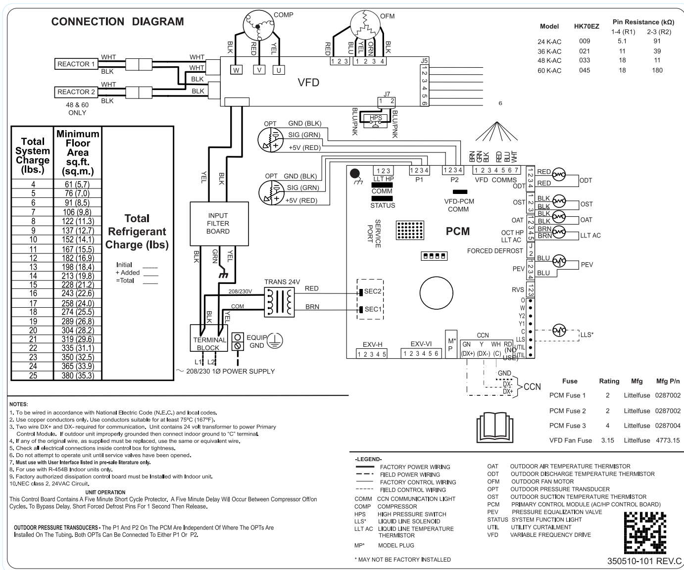
Fig. 1 – Size 2 - 5 Tons
