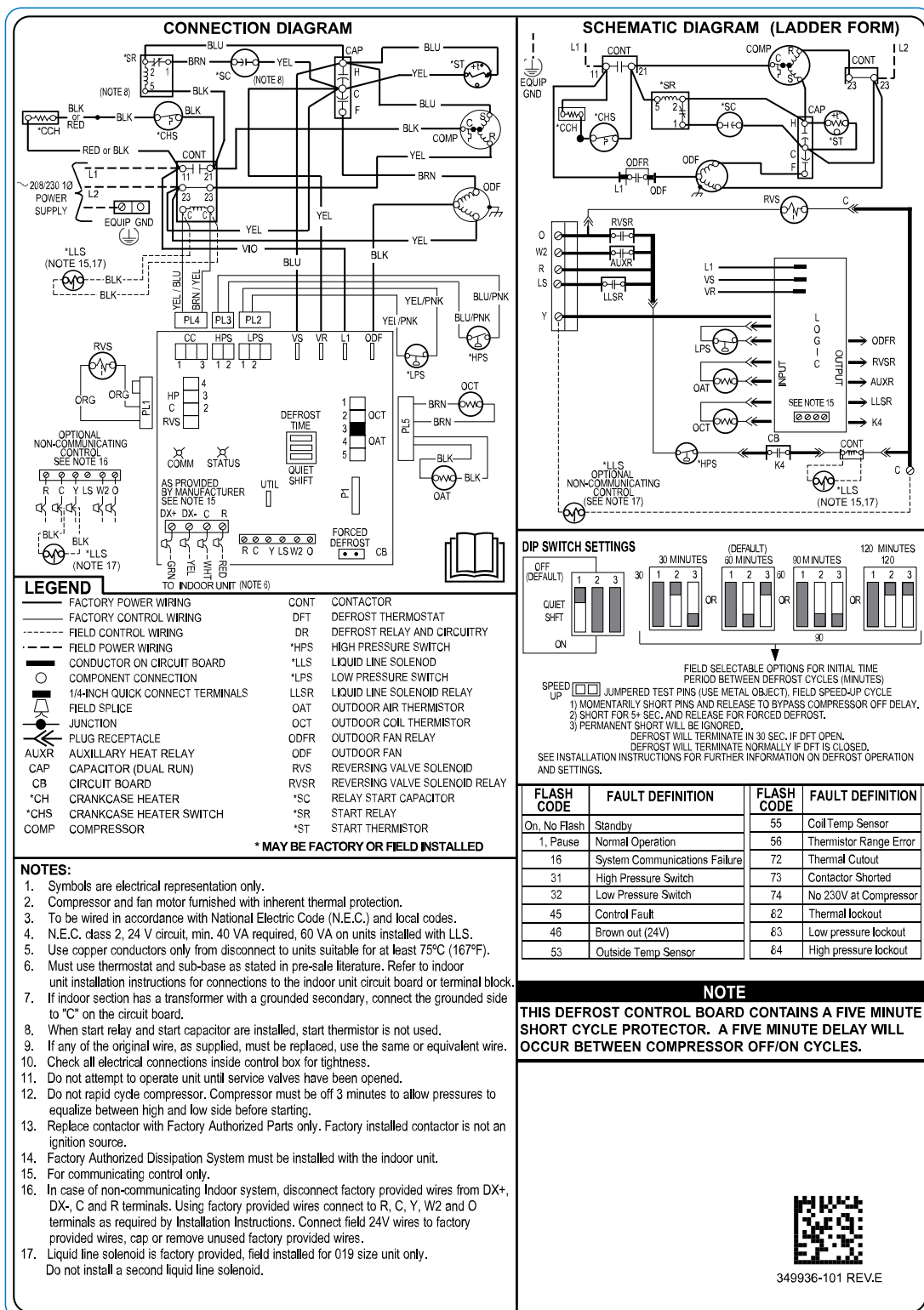
Fig. 1 – Size 1.5 - 5 Tons
