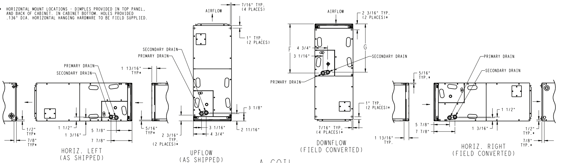
Fig. 6 – FX4DNB - English
