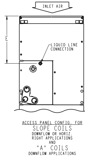
Fig. 1 – FX4DNF - English
