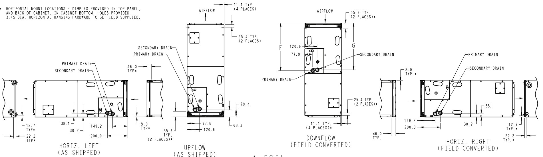
Fig. 8 – FX4DNB - Metric
