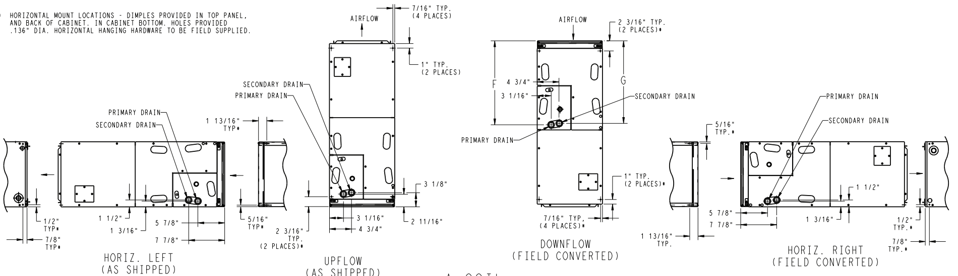
Fig. 2 – FX4DNF - English
