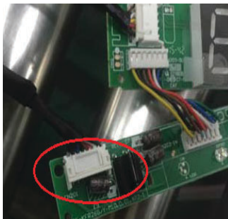
Fig. 18 — CN201 Connection to the Main Control Board
