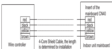
Fig. 3 — Wiring Connection Diagram
