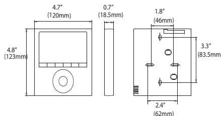
Fig. 2 — Wired Remote Controller Dimensions
