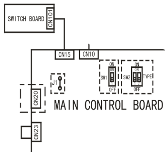
Fig. 28 — Main Control Board
