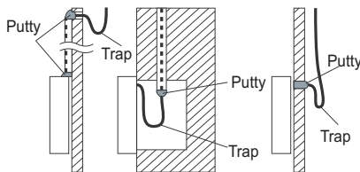
Fig. 12 — Seal the wires
