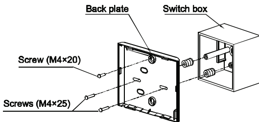
Fig. 7 — Flush Mounting
