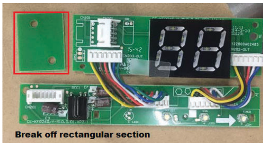
Fig. 21 — Display Board
