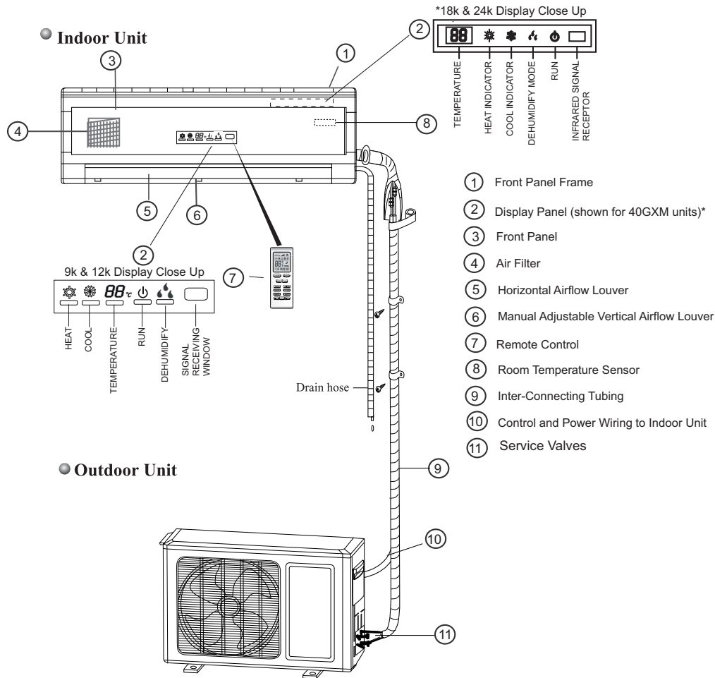
Indoor/Outdoor Unit
