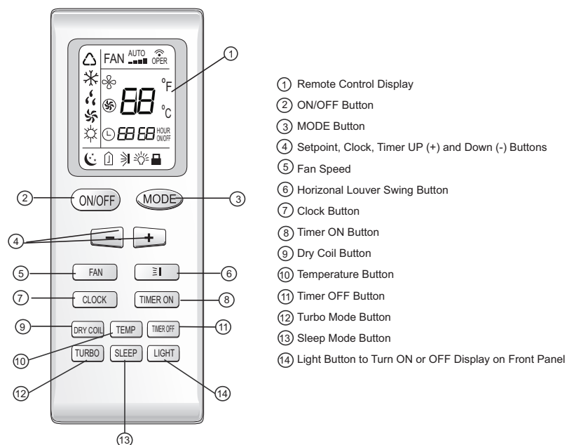
Remote Control
