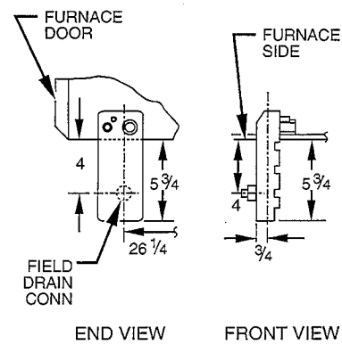
HORIZONTAL APPLICATIONS
