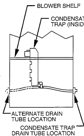
UPFLOW APPLICATIONS
