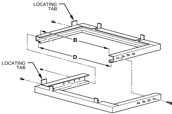
Disassembled
