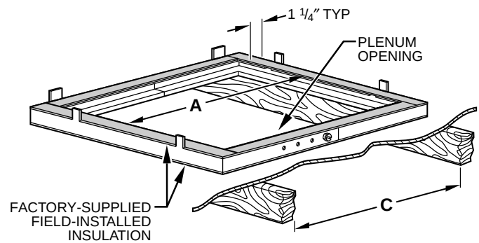
Assembled
