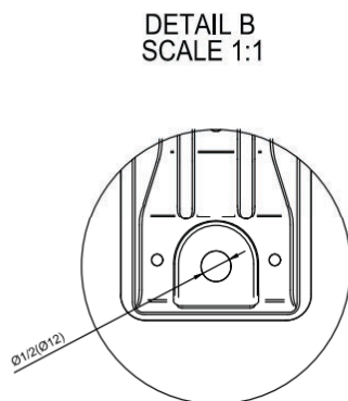
Fig. 5 – Sizes 30 and 36K, in. (mm)
