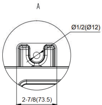
Fig. 6 – Sizes 48 and 55K, in. (mm)
