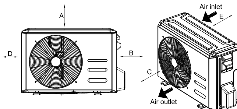
Fig. 7 — Clearances
