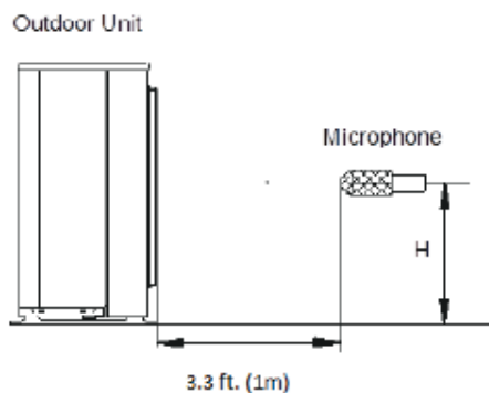
Fig. 9 – Outdoor Unit Sound Pressure Test Conditions
