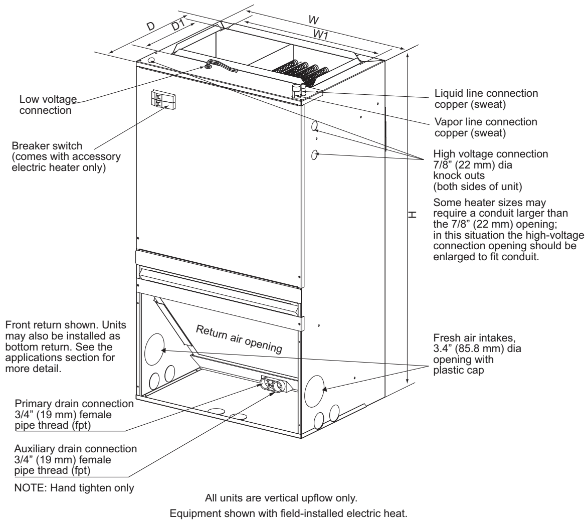
Fig. 1 - Dimensional Drawing with Circuit Breaker
