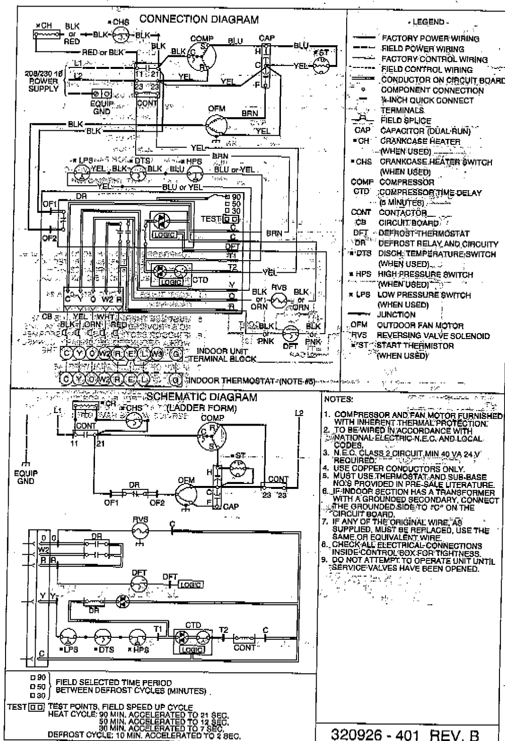
Fig. 1—693C024-048 208/230v, 1 Phase, 60 Hertz
