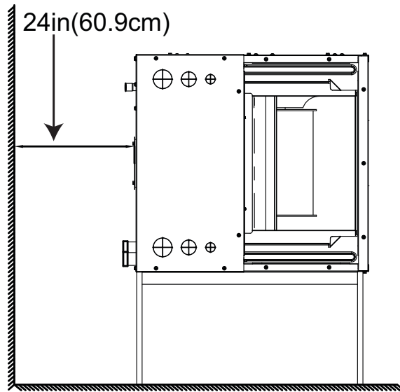
Horizontal Installations
