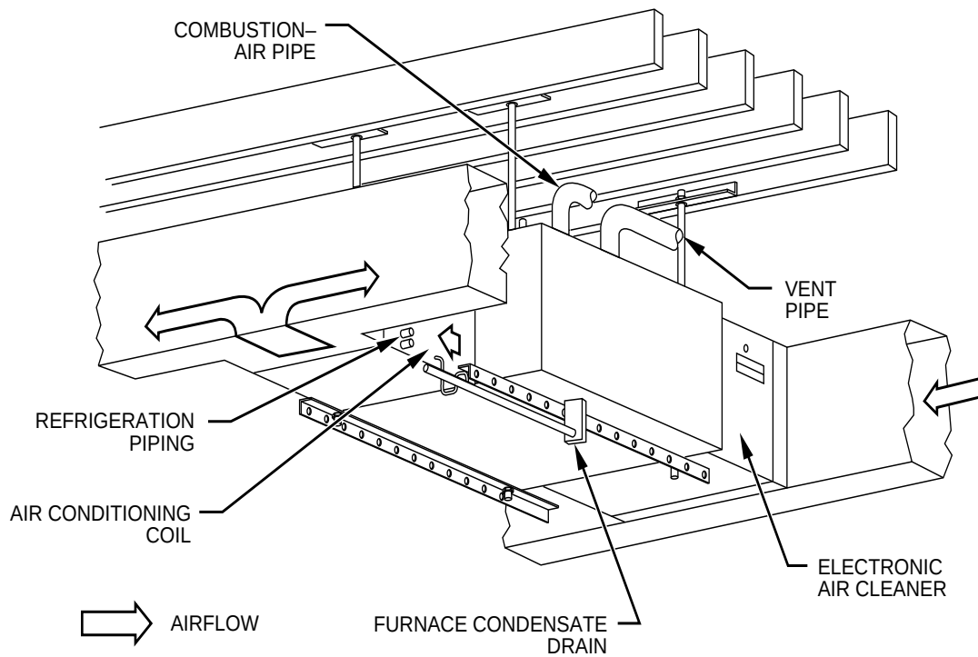
Crawlspace — Horizontal Application
