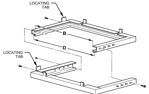
Disassembled
