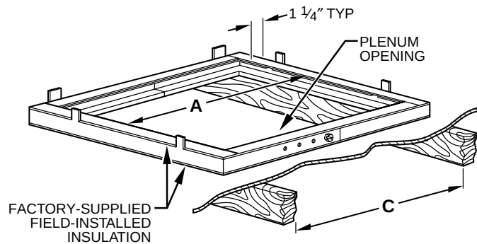
Assembled
