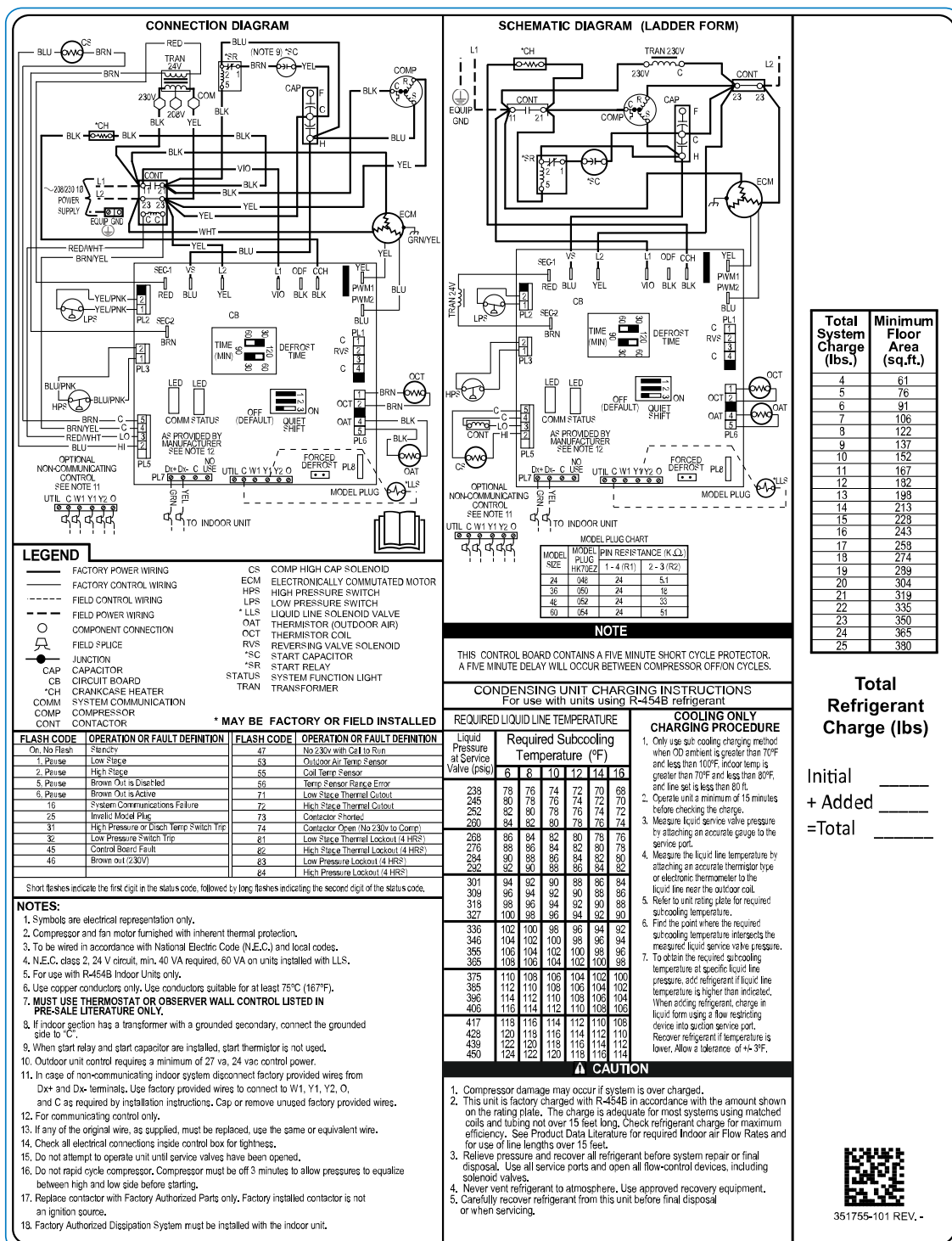
Fig. 1 – Size 2 through 5 Tons
