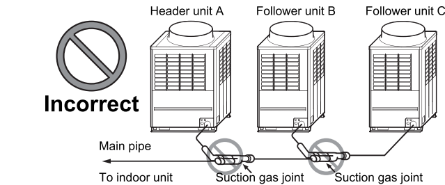
<Suction gas joint reverse orientation installation> Figure 4
