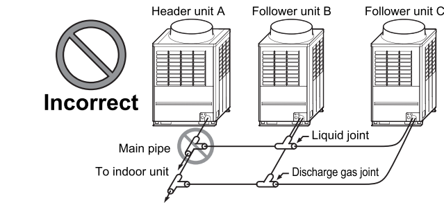
Suction gas pipes Figure 3
