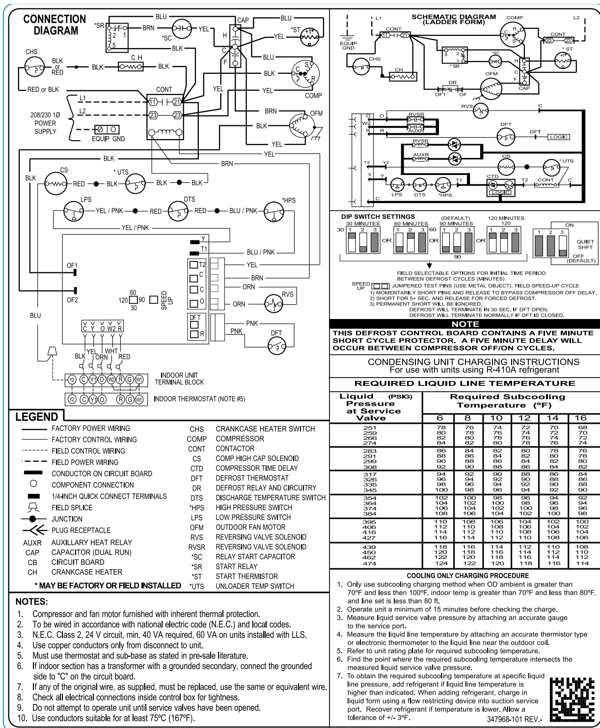
Fig. 1 – 208/230-1 - Model Sizes 24 - 60
